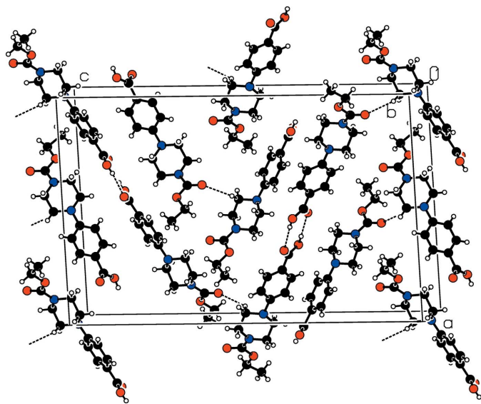
Figure 2 Part of the crystal structure with O—H···O and weak C—H···O hydrogen bonds shown as dashed lines.
