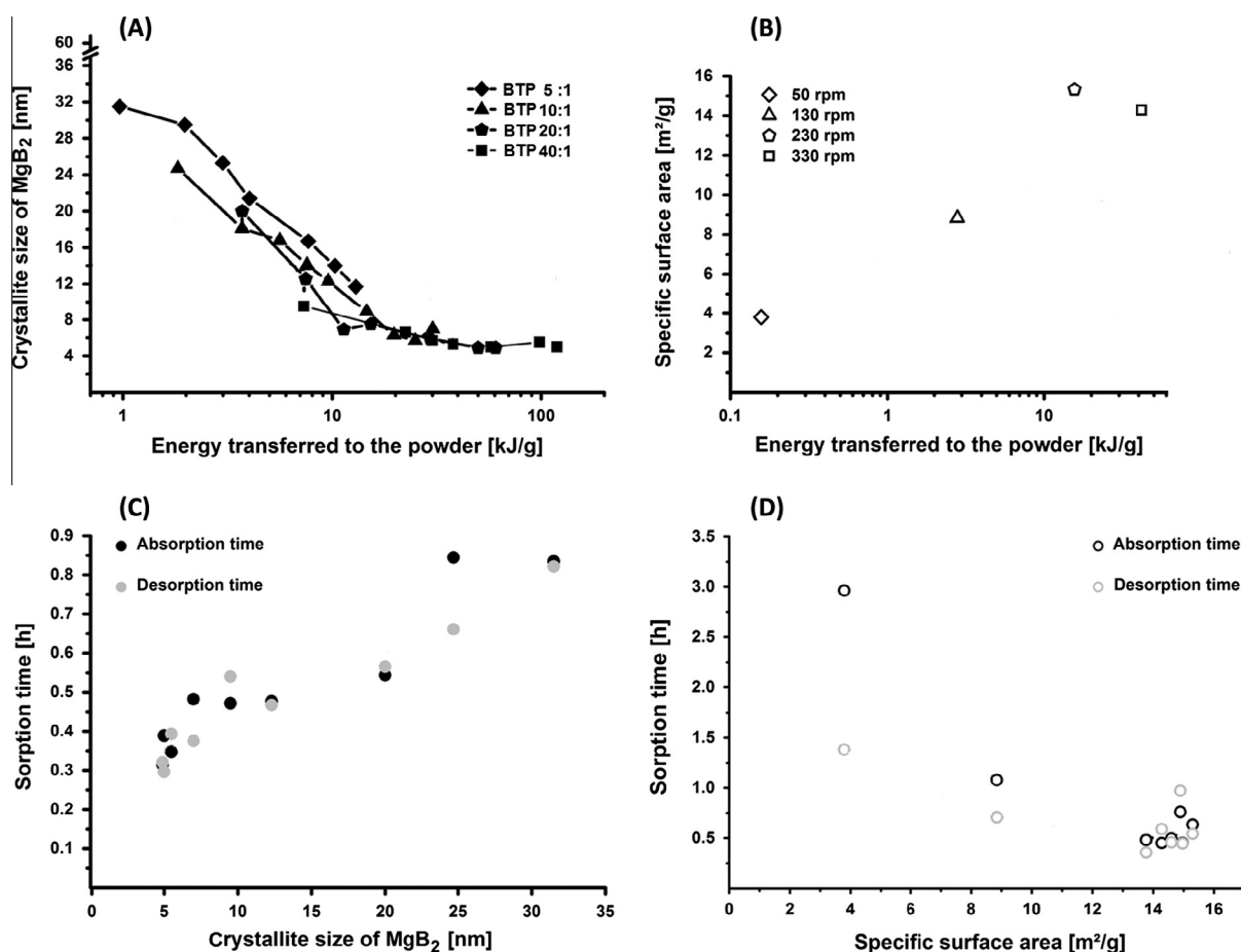
Fig. 2. (A) Crystallite size of \text{MgB}_2 and (B) specific surface area as a function of the energy transferred to the powder. Sorption times changes with (C) crystallite size of \text{MgB}_2 and (D) specific surface area.
