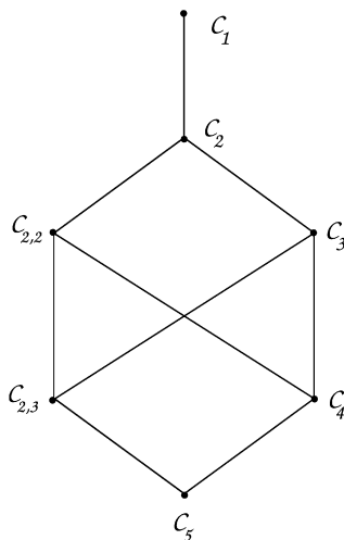
Fig. 1. The conjugacy graph \Gamma(S_5, \{C_2\}) , where the vertices C_1, C_2, C_3, C_4, C_5, C_{2,2}, C_{2,3} are the conjugacy classes of e_{S_5}, (1, 2), (1, 2, 3), (1, 2, 3, 4), (1, 2, 3, 4, 5), (1, 2)(3, 4), (1, 2)(3, 4, 5) respectively.
