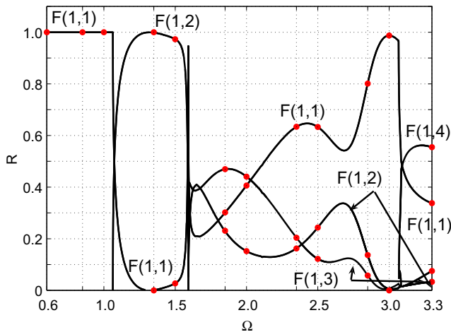
Fig. 6. Power reflection coefficients of flexural modes when the F(1,1) mode encounters a free-end cylinder. The bullets (•) are results found in Taweel et al. (2000).
