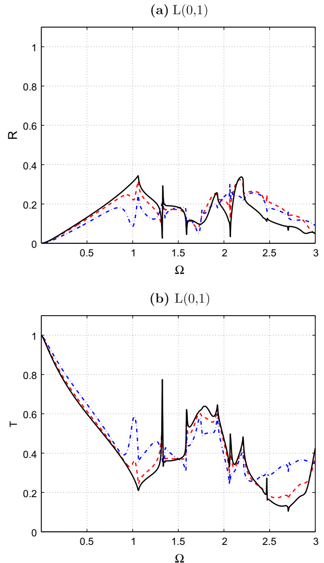
Fig. 15. Power reflection (a) and transmission (b) coefficients of the compressional mode L(0,1) when it encounters a d = 1.0r crack depth of angle 0^\circ (—), 10^\circ (— · —) and 20^\circ (---).
