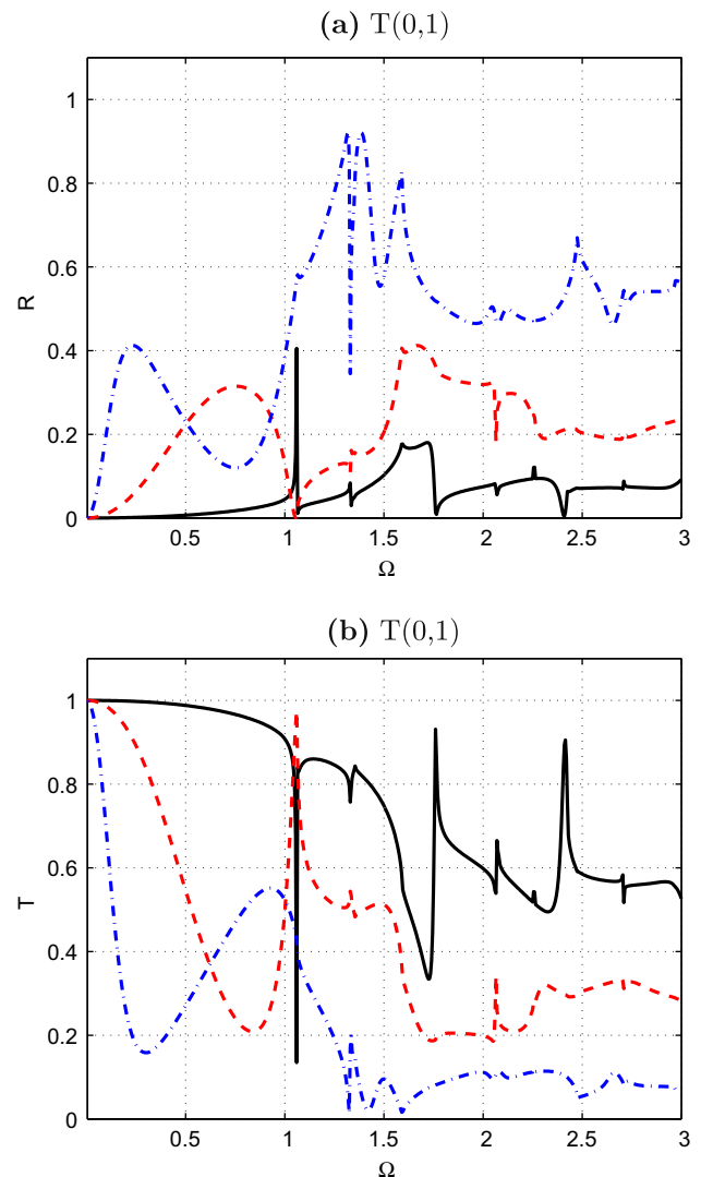
Fig. 9. Power reflection (a) and transmission (b) coefficients of the torsional mode T(0,1) when it encounters a crack with depths d = 0.5r (—), d = 1.0r (---) and d = 1.5r (- · -).
