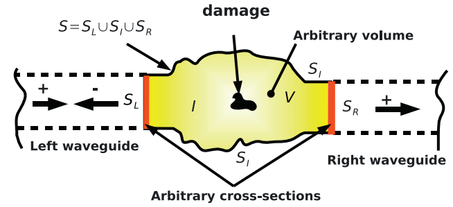
Fig. 1. Description of the problem in the case of a damaged volume located between two semi-infinite waveguides (2D representation).
