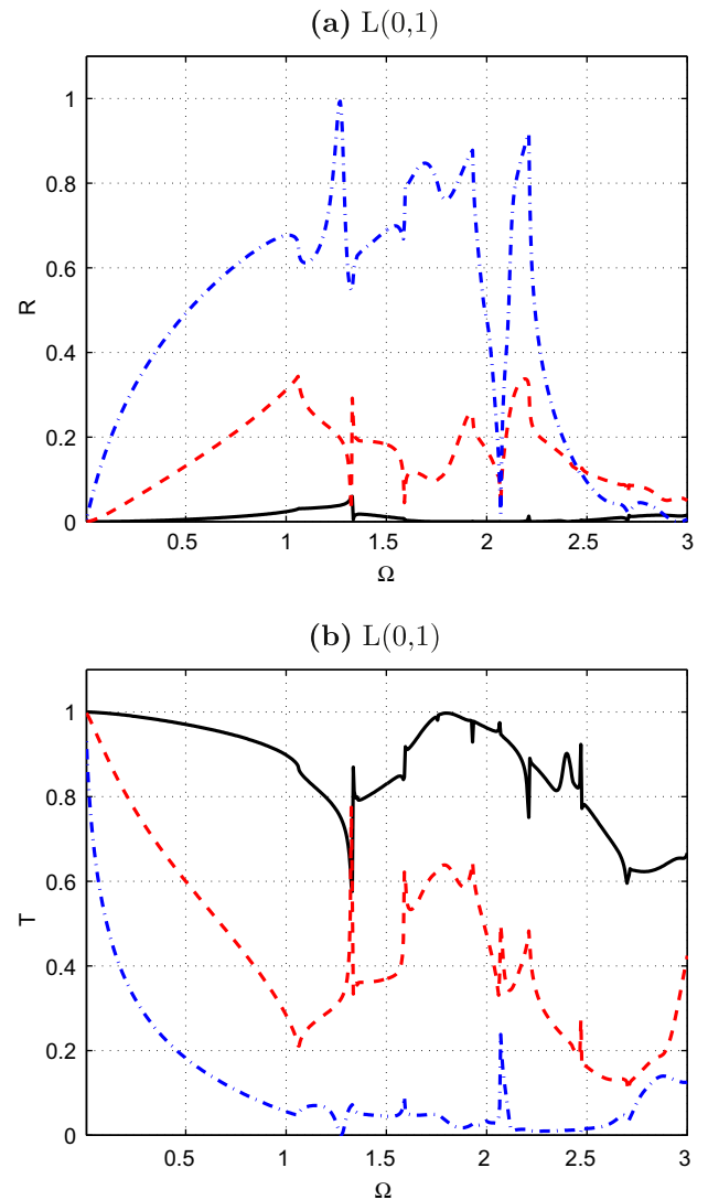
Fig. 7. Power reflection (a) and transmission (b) coefficients of the compressional mode L(0,1) when the L(0,1) mode encounters a crack with depths d = 0.5r (—), d = 1.0r (---) and d = 1.5r (···).
