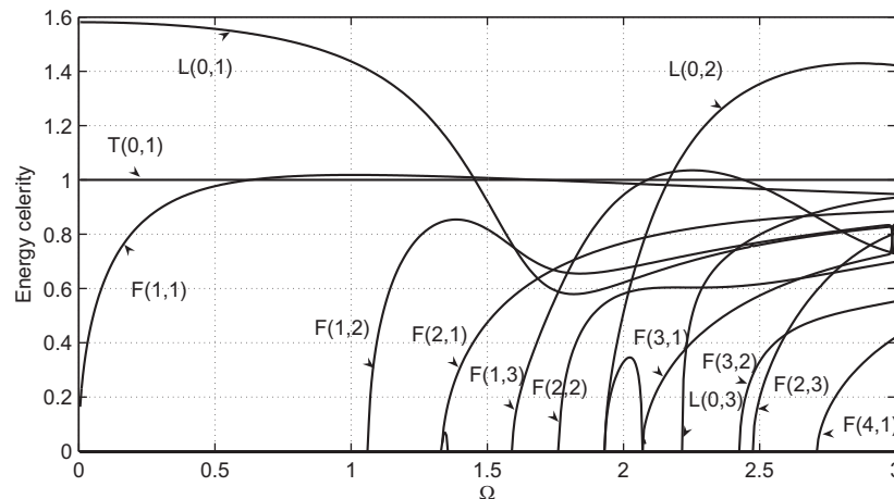
Fig. 4. Dispersion curves of dimensionless energy velocity versus dimensionless frequency.
