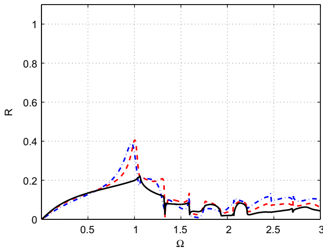
Fig. 16. Power reflection coefficients of the flexural mode F(1,1) when the L(0,1) mode encounters a d = 1.0r crack depth of angle 0^\circ (—), 10^\circ (---) and 20^\circ (- · -).
