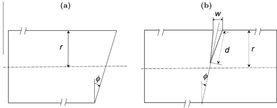
Fig. 13. Description of an oblique free-end cylinder (a) and an oblique crack (b).
