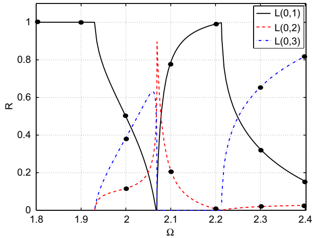
Fig. 5. Power reflection coefficients of compressional modes L(0,1) (—), L(0,2) (---) and L(0,3) (···) when the L(0,1) mode encounters a free-end cylinder. The bullets (•) are results found in Gregory and Gladwell (1989).
