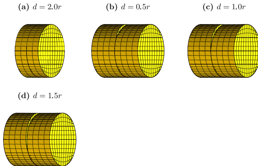
Fig. 3. Meshing of a cylinder with a free-end of d = 2.0r (a) and vertical cracks of depths of 0.5r (b), 1.0r (c) and 1.5r (d).
