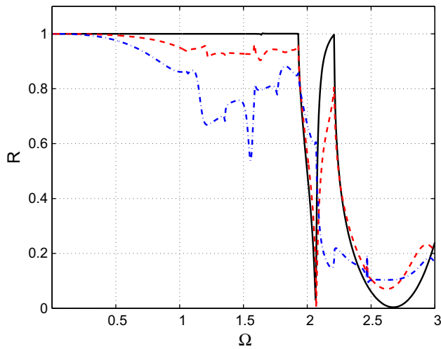
Fig. 14. Power reflection coefficients of the compressional mode L(0,1) when it encounters a free-end cylinder of angle 0^\circ (—), 10^\circ (— · —) and 20^\circ (---).
