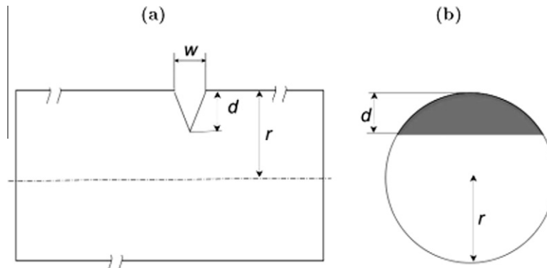
Fig. 2. Description of a vertical non-axisymmetric crack: side view (a) and cross-section view (b).
