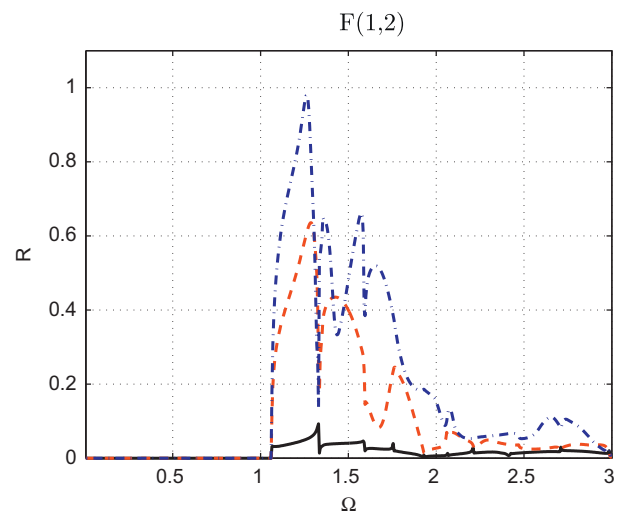
Fig. 12. Power reflection coefficient of the flexural mode F(1,2) when the F(1,1) mode encounters a crack with depths d = 0.5r (—), d = 1.0r (---) and d = 1.5r (— ·).
