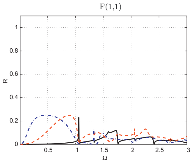
Fig. 10. Power reflection coefficient of the flexural mode F(1,1) when the T(0,1) mode encounters a crack with depths d = 0.5r (—), d = 1.0r (---) and d = 1.5r (— ·).
