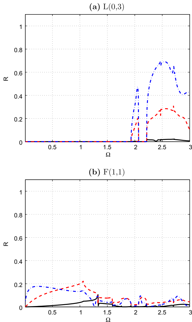
Fig. 8. Power reflection coefficient of the L(0,3) (a) and F(1,1) (b) modes when the L(0,1) mode encounters a crack with depths d = 0.5r (—), d = 1.0r (---) and d = 1.5r (- · -).
