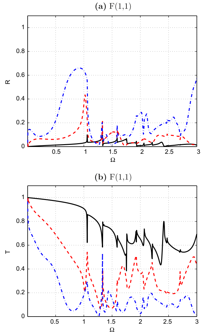
Fig. 11. Power reflection (a) and transmission (b) coefficients of the flexural mode F(1,1) when the F(1,1) mode encounters a crack with depths d = 0.5r (—), d = 1.0r (---) and d = 1.5r (— ·).
