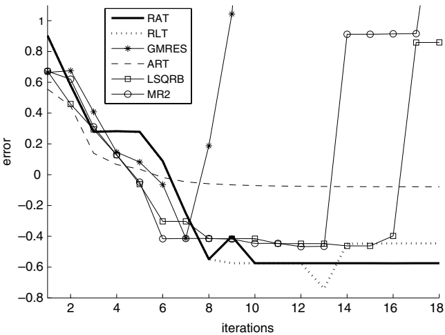
Fig. 4. Error behavior for SHAW(64) with noise. RAT and RLT are implemented with \lambda = 100 .
