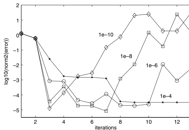
Fig. 2. BAART(120)—Error behavior for \lambda = 10^{-4}, 10^{-6}, 10^{-8}, 10^{-10} .
