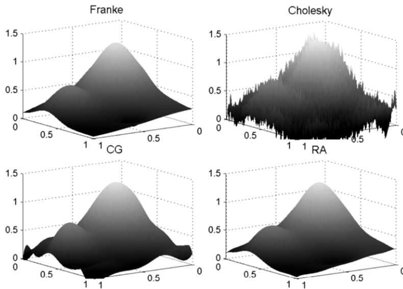
Fig. 3. Interpolation of Franke's bivariate test function by means of Gaussian RBF.
