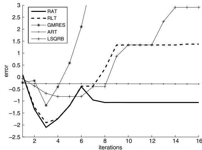
Fig. 5. Error behavior for BAART(120) with noise. RAT and RLT are implemented with \lambda = 100 .
