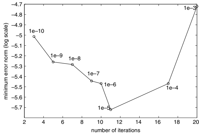
Fig. 1. BAART(40)—Minimum attained error with respect to the number of iterations for different values of \lambda .
