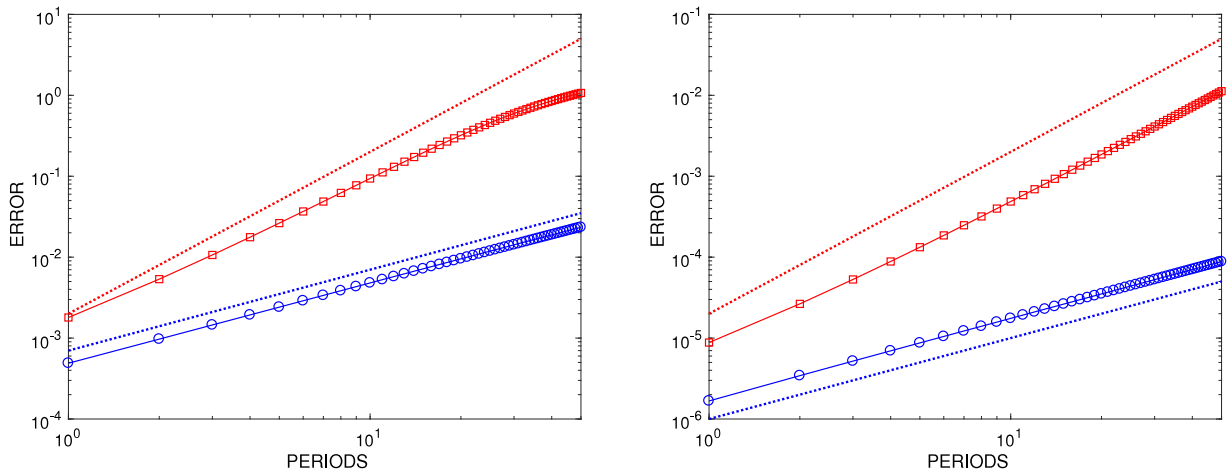
Fig. 1. Poisson problem (87)–(90). Left-plot: solution error along 50 periods for EQUIP(6,2) (circles and solid line) and GAUSS2 (squares and solid line). Right-plot: solution error along 50 periods for EQUIP(6,3) (circles and solid line) and GAUSS2 (squares and solid line). In both plots, the linear and quadratic grows are reported in dotted-line.
