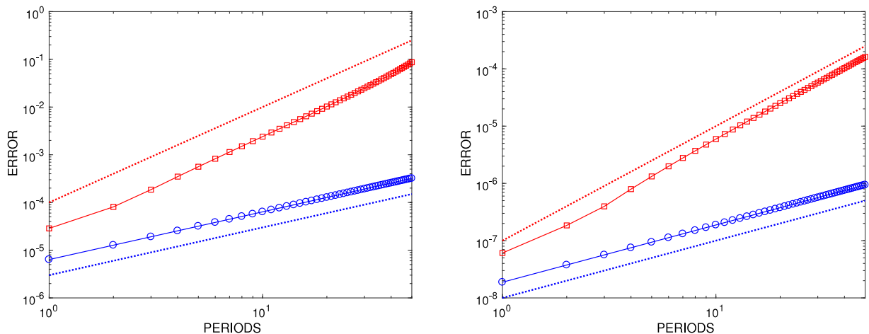
Fig. 2. Lotka-Volterra problem (91)–(92). Left-plot: solution error along 50 periods for EQUIP(6,2) (circles and solid line) and GAUSS2 (squares and solid line). Right-plot: solution error along 50 periods for EQUIP(6,3) (circles and solid line) and GAUSS2 (squares and solid line). In both plots, the linear and quadratic grows are reported in dotted-line.
