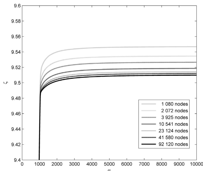
Fig. 4. Loading paths for \alpha \in [0, 10\,000] (zoom).
