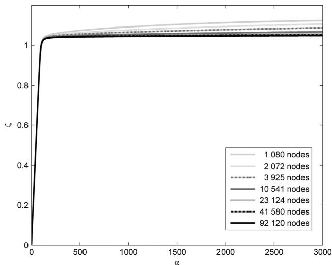
Fig. 5. Loading paths up to \alpha = 3000 .
