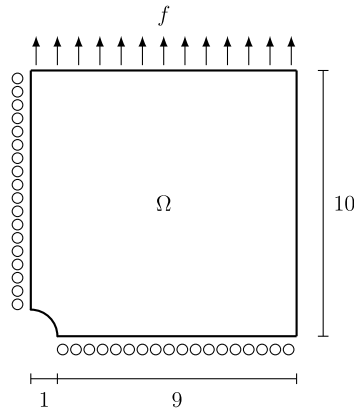
Fig. 2. Geometry of the plane strain problem.
