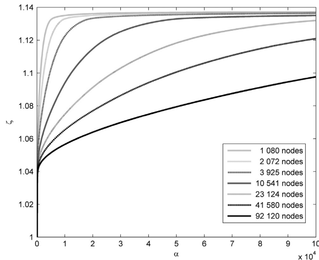
Fig. 6. Loading paths up to \alpha = 100\,000 (zoom).
