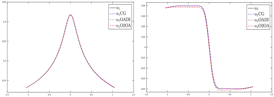
Figure 1: First test: The reconstructed velocity on \Gamma_I with \epsilon = 0 .
