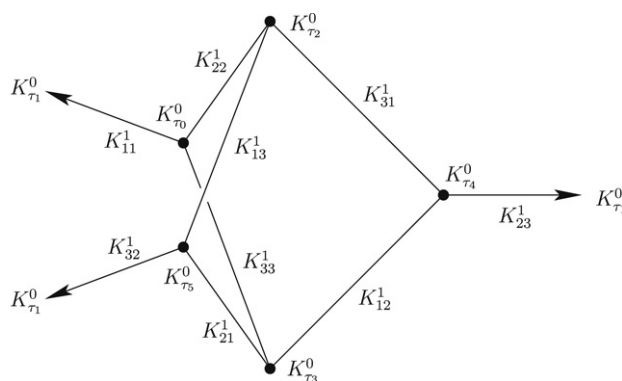
Fig. 1. The subcomplex of the 2-skeleton consisting of cells that do not intersect K_{\tau_1}^0 . The 2-cells form the faces of the triangular double pyramid.
