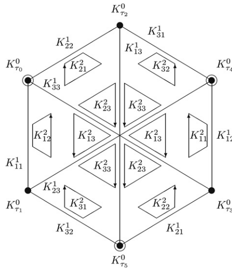
Fig. 2. The 2-skeleton of Y with orientation. The starting points of the 1-cells are encircled. The orientations of the 2-cells are indicated by an arrow along the boundary of the corresponding symbols. Note that the crossing point at the center is not a vertex.
