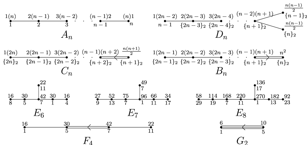
Fig. 3. The lengths L(t_i) and Coxeter exponents m_i for all Dynkin graphs.
