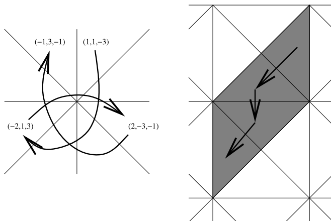
Fig. 2. The graph \Gamma(W_0^j) in B_2 , and the unit hypercube in \tilde{B}_2 .
