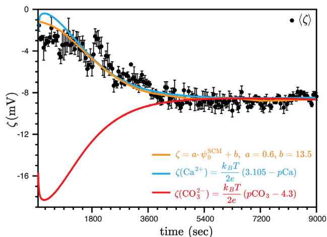
Fig. 4. Measured (black dots) and calculated (solid lines, Eqs. (6)–(8)) time-evolution of the electrokinetic potential.
