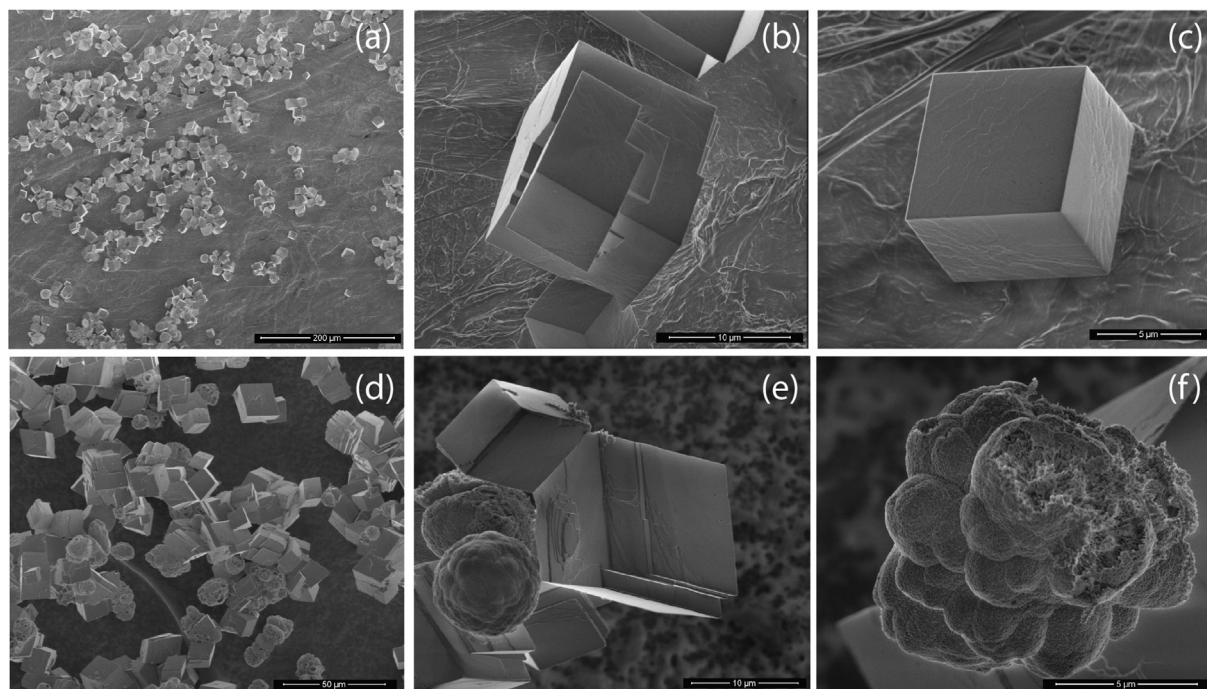
Fig. 3. Scanning electron microscopy (SEM) micrographs taken two hours after the reagents were mixed and showing the presence of the calcite (rhombohedral morphology, a–c) and vaterite (spherulitic morphology, d–f) particles.
