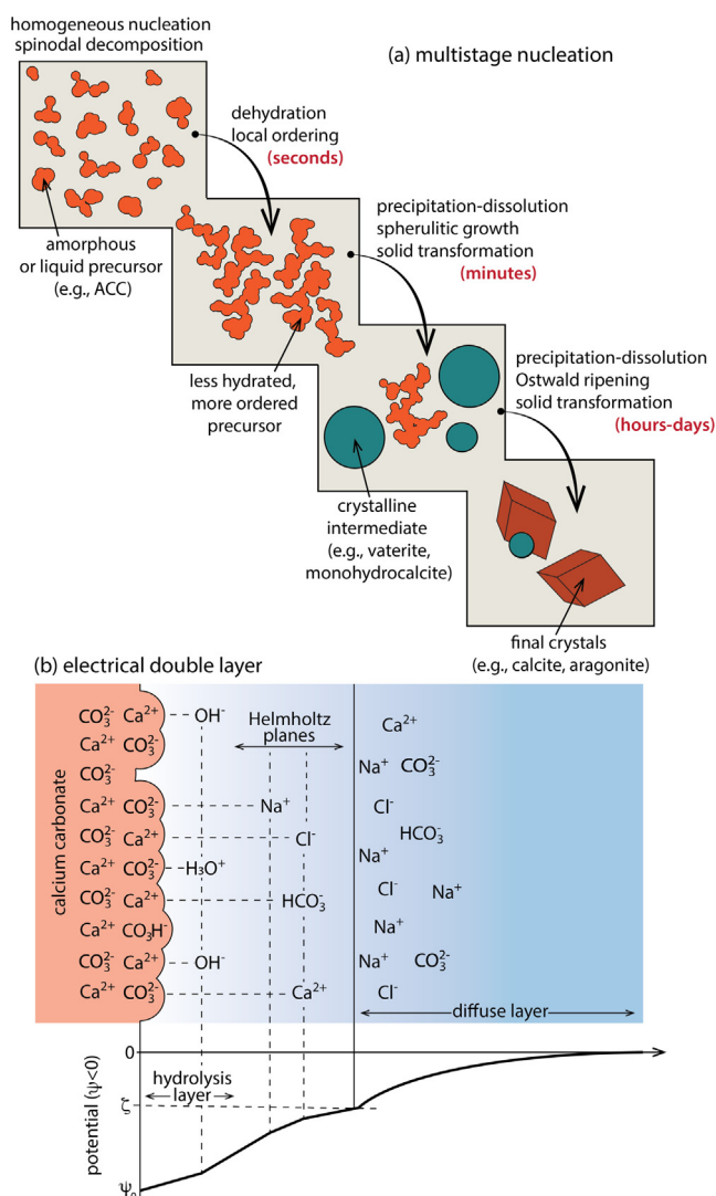
Fig. 1. Schematic representation of the multistage nucleation pathway of \text{CaCO}_3 (a): (i) formation of amorphous calcium carbonate (ACC) or polymeric liquid precursors [2,11–17], (ii) dehydration and local ordering [21–26] (iii) precipitation-dissolution transformation or spherulitic growth [28–33], and finally (iv) formation of the most stable \text{CaCO}_3 mineral. In Panel (b) we show a schematic diagram of the electrical double layer formed at the carbonate/NaCl-electrolyte interface. The surface charge is defined by constituent ions at the surface and their hydrolysis products [34,35]. The electrokinetic potential ( \zeta ) quantifies the electrostatic potential at the slip plane in the diffuse part of the electrical double layer.
