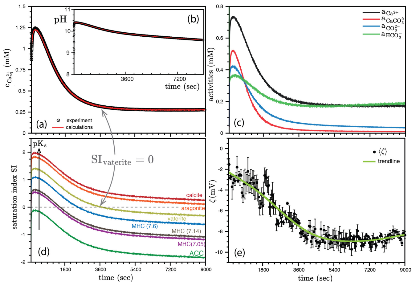
Fig. 2. Comparison between experimental and calculated values of the averaged \text{Ca}^{2+} concentration and bulk pH time evolution between 70 and 9000 s after the reagents are mixed (a, b). In panels c, d we show the calculated evolution of aqueous speciation (c) and saturation indexes (d) obtained from the time-resolved speciation code. The electrokinetic potential (e) was obtained in a separate set of experiments using time-resolved electrophoretic cell ( \zeta = -8.62 mV after 24 h). The green solid line illustrates the trend of the \zeta -evolution and the error bars represent a standard error from three independent measurements.
