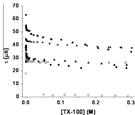
Fig. 4. Titration curves from lifetime vs. [TX-100] for all \text{Cr}(\text{NN})_3^{3+} complexes in 0.1 M NaCl at pH=2 (HCl) at 25 \pm 0.5 °C: ■ ( \text{Cr}(\text{5Clphen})_3^{3+} ); ▲ ( \text{Cr}(\text{bpy})_3^{3+} ); ● ( \text{Cr}(\text{phen})_3^{3+} ); ○ ( \text{Cr}(\text{Ph}_2\text{phen})_3^{3+} ); □ ( \text{Cr}(\text{Me}_4\text{phen})_3^{3+} ) and * ( \text{Cr}(\text{Me}_2\text{phen})_3^{3+} ).
