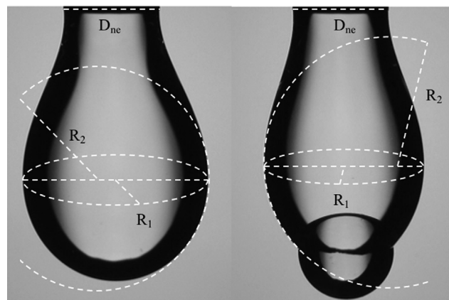
Fig. 2. Illustration of the curvature radii measurement for a single pendant drop (left) and a loaded pendant drop with a glass bead (right).
