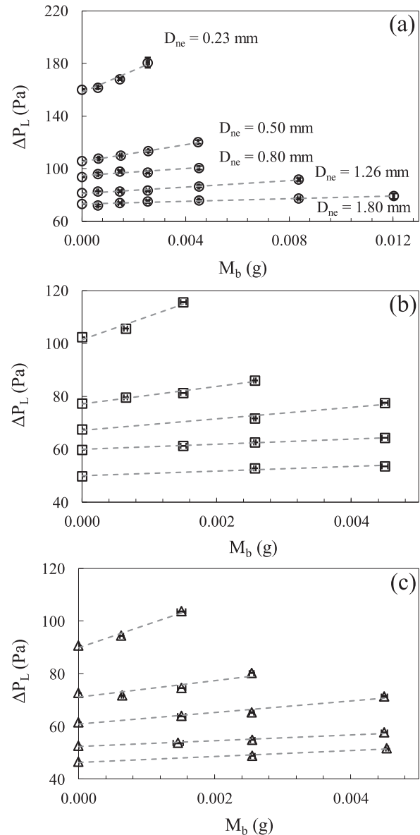
Fig. 7. Laplace pressure within the maximal pendant drops as a function of the particle mass for (a) Water, (b) Tween 80, (c) Triacetin and different external diameters of the needle ( D_{ne} = 0.23, 0.50, 0.80, 1.26 and 1.80 mm). The order of the diameters is respected for each figure. The dashed lines are a guideline.
