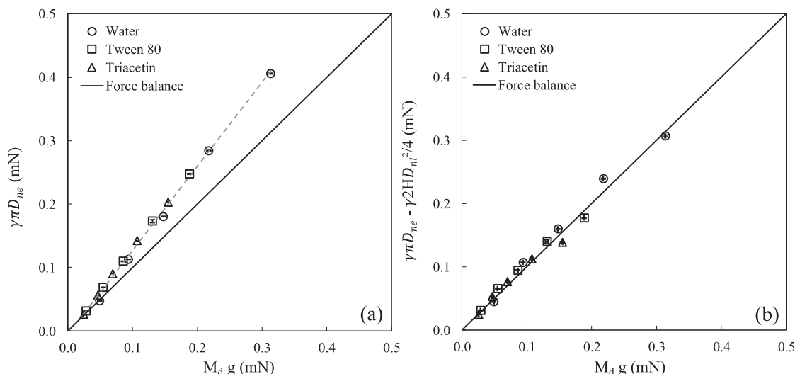
Fig. 3. (a) Capillary force as a function of the maximal drop weight (Eq. (2)) for all experiments, (b) capillary force minored by the “Laplace force” versus maximal drop weight (Eq. (4)) for all experiments. The order of the error magnitude is about 10^{-4} mN. The dashed line is a guideline.
