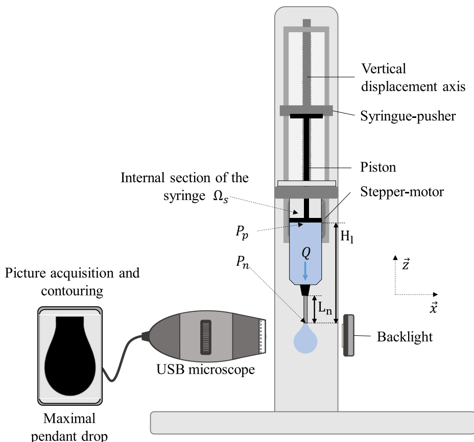
Fig. 1. Scheme of the experimental prototype for pendant drop generation and contouring acquisition of the maximal pendant drop.
