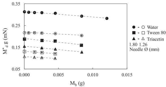
Fig. 5. Maximal mass of loaded pendant drops as a function of bead mass for Water (circle), Tween 80 (square) and Triacetin (triangle). For each liquid only results, obtained for needles of external diameters equal to 1.26 (empty symbols) and 1.80 mm (blank symbols), are shown. The dashed lines are a guideline. Full results are available in the Supplementary Materials file.
