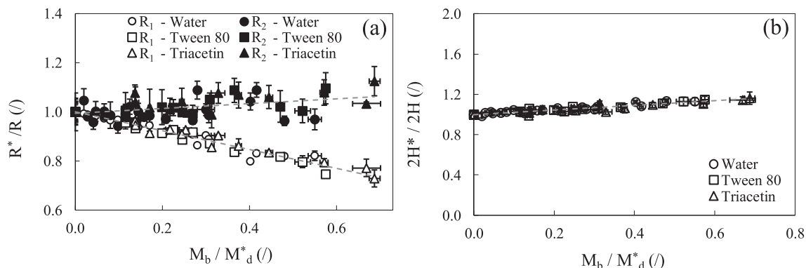
Fig. 6. Variation of the loaded pendant drop curvatures as a function of the solid mass fraction for all experiments: (a) dimensionless curvature radii, (b) dimensionless mean curvature. The dashed lines are a guideline.
