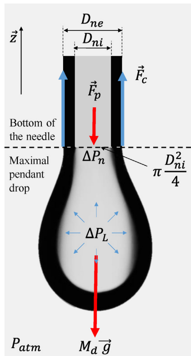
Fig. 9. Scheme of the external forces applied to a maximal pendant drop generated by a syringe.
