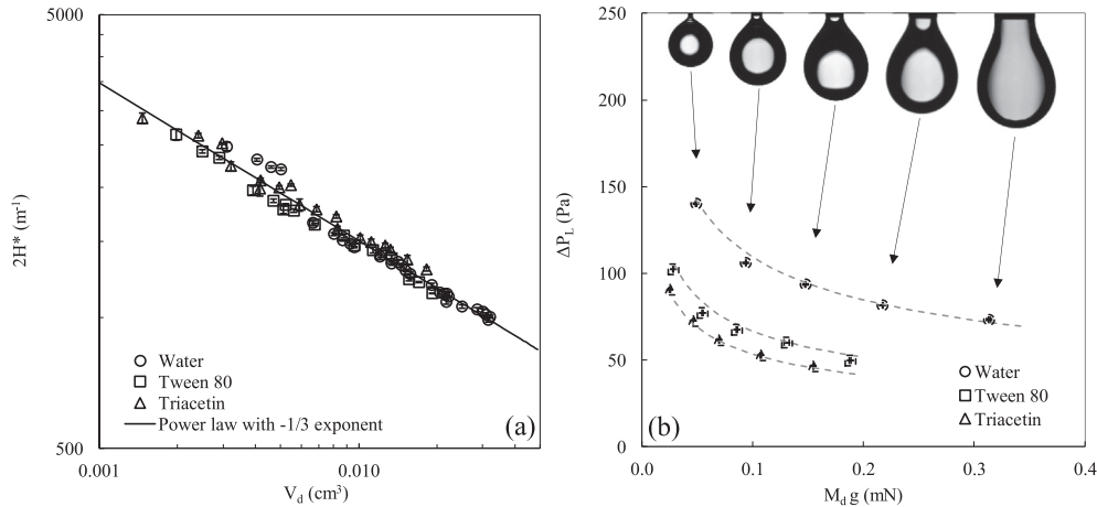
Fig. 8. (a) Variation of the mean curvature as a function of the maximum pendant drop volume ( R^2 = 0.9736 ) for all liquids and needles used (Log-Log representation), (b) Laplace pressure within the maximal pendant drops as a function of its weight.
