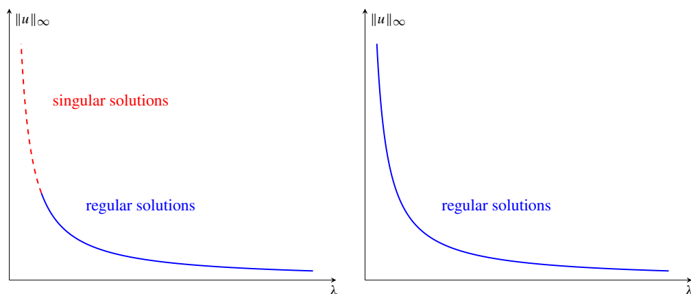
Fig. 2. Global bifurcation diagrams in case p > 2 when (a_2) holds (on the left), or (a_2) fails (on the right).
