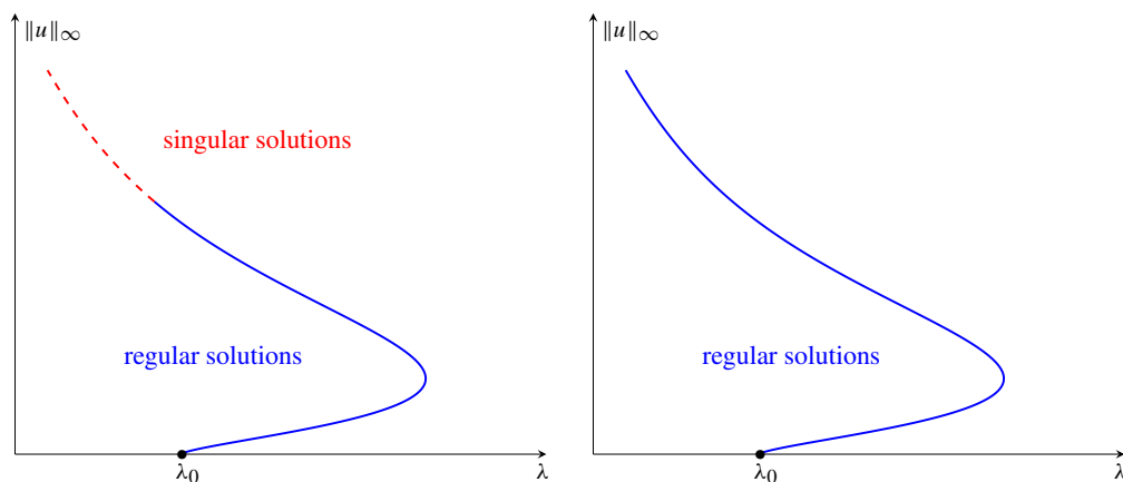
Fig. 1. Global components emanating from the positive principal eigenvalue \lambda_0 in case p = 2 when (a_2) holds (on the left), or (a_2) fails (on the right).
