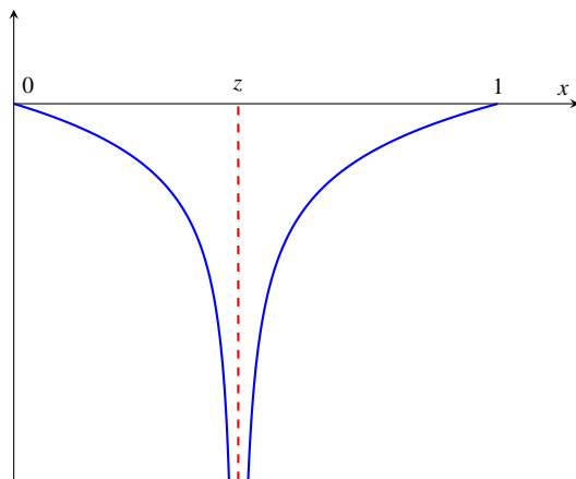
Fig. 3. Profile of the limiting derivative u'_\omega .
