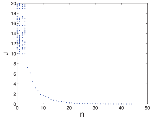
FIGURE 6. Convergence results - evolution of the functional J during the optimization procedure.
