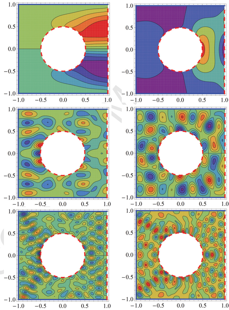
FIGURE 4. first components (left plots) and second components (right plots) of the eigenfunction associated to \Lambda_1 \approx 2.91741 , \Lambda_{100} \approx 289.41906 and \Lambda_{600} \approx 1066.68372 .
