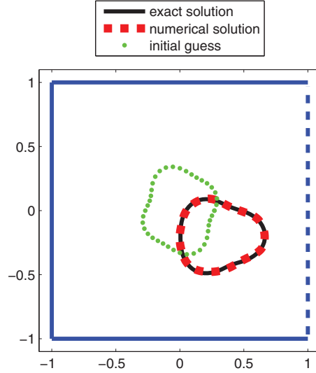
FIGURE 5. The target hole \tilde{V} (continuous black line), the initial guess (green dots) and the computed hole V (red dashed line).
