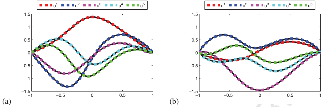
FIGURE 7. (a) first components of the target \tilde{u}^q|_{\Gamma_N} (continuous black line) and u^q|_{\Gamma_N} (dashed lines), for q = 1, \dots, 5 ; (b) similar results for the second component of the eigenfunctions.
