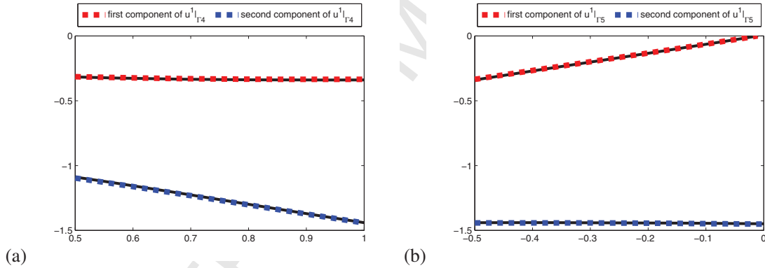
FIGURE 11. (a) first and second components of the target \tilde{u}^1|_{\Gamma_4} (continuous black line), first component of u^1|_{\Gamma_4} (dashed red line) and second component of u^1|_{\Gamma_4} (dashed blue line); (b) similar results on \Gamma_5 .
