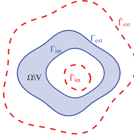
FIGURE 2. The boundaries \Gamma_{int} and \Gamma_{ext} and the artificial boundaries \hat{\Gamma}_{int} and \hat{\Gamma}_{ext} .
