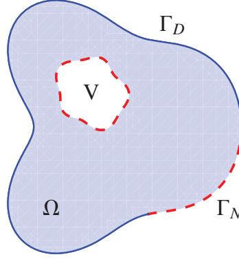
FIGURE 1. The boundaries for the problem of detecting an inclusion V .
