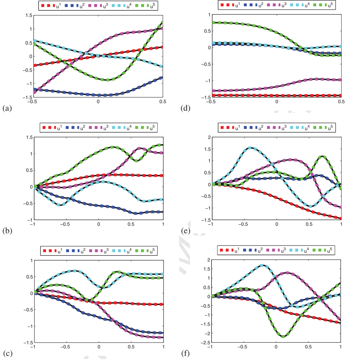
FIGURE 9. (a) first components of the target \tilde{u}^q|_{\Gamma_1} (continuous black line) and of the numerical approximation u^q|_{\Gamma_1} (dashed lines); (b) first components of \tilde{u}^q|_{\Gamma_2} (continuous black line) and u^q|_{\Gamma_2} (dashed lines); (c) first components of \tilde{u}^q|_{\Gamma_3} (continuous black line) and u^q|_{\Gamma_3} (dashed lines); (d) (e) (f) similar results for the second components of the eigenfunctions.
