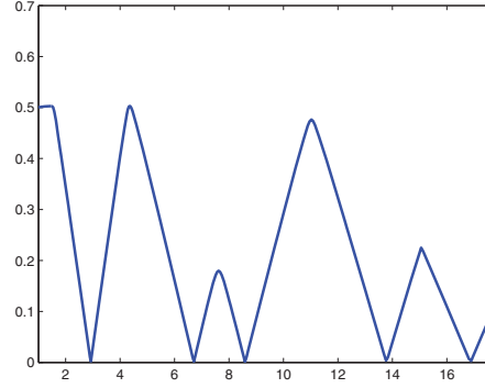
FIGURE 3. \sigma_1(\Lambda) for \Lambda \in [1, 17.5] .
