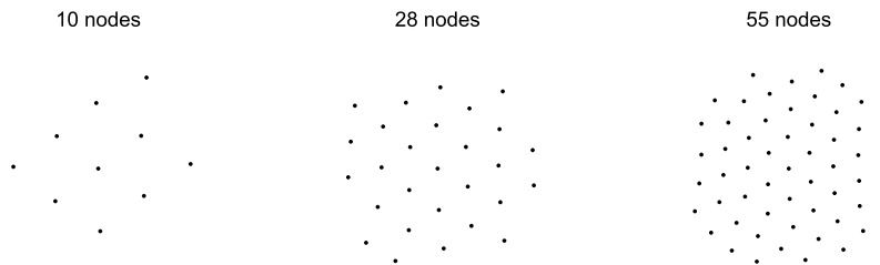
Fig. 13. The three different stencils used for approximation of (12). In all cases, the error is calculated over evaluation points near the stencil center.
