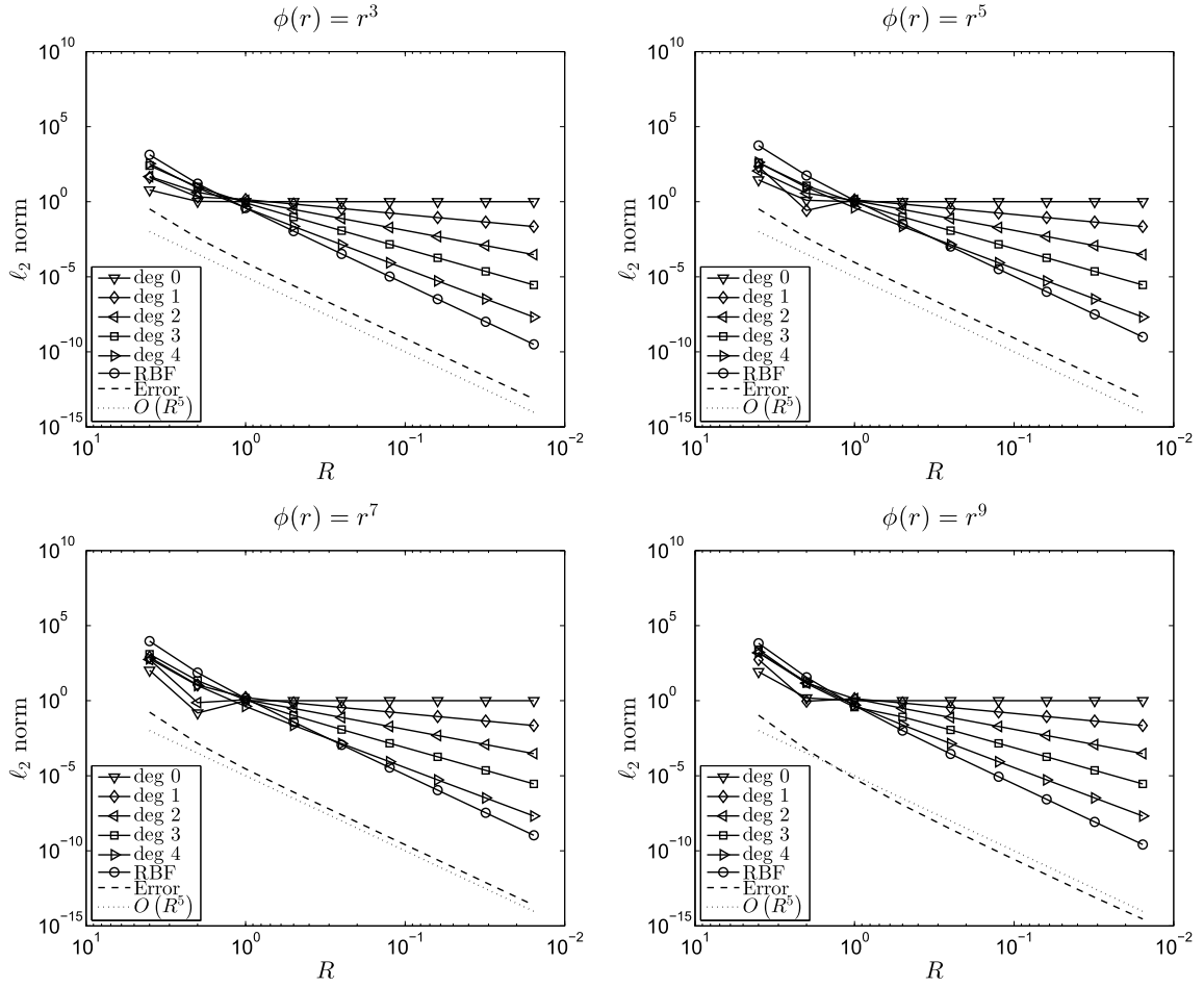
Fig. 8. Behavior of the PHS and polynomial coefficients under refinement, where the latter have been separated according to polynomial degree. For the RBFs r^3 , r^5 , r^7 , and r^9 , the condition numbers of the collocation matrix are 3 \times 10^4 , 5 \times 10^5 , 5 \times 10^6 , and 3 \times 10^7 , respectively. In every case, the RBF coefficients converge to zero at the same rate as the interpolation error.
