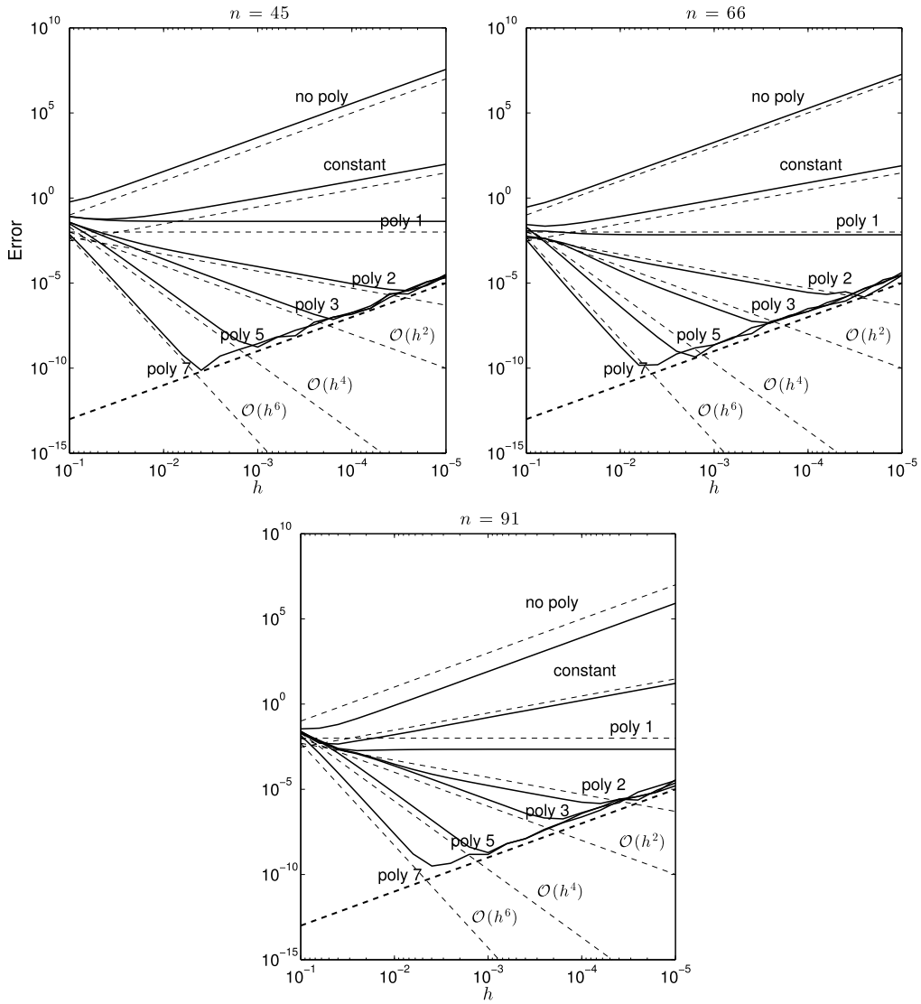
Fig. 12. The worst error encountered when approximating the Laplacian of (12) using RBF-FD stencils based on r^7 + polynomials as described in the text. The thin dashed lines represent the convergence order O(h^{l-k+1}) for each polynomial order l . Notice that the convergence rate is independent of the stencil size and only depends on the degree of polynomial terms included. Only for polynomial up to degree two do we see any clear accuracy gain with stencil size. As in the previous figure, the thick dashed line marks the round-off limit 10^{-15}/h^2 .
