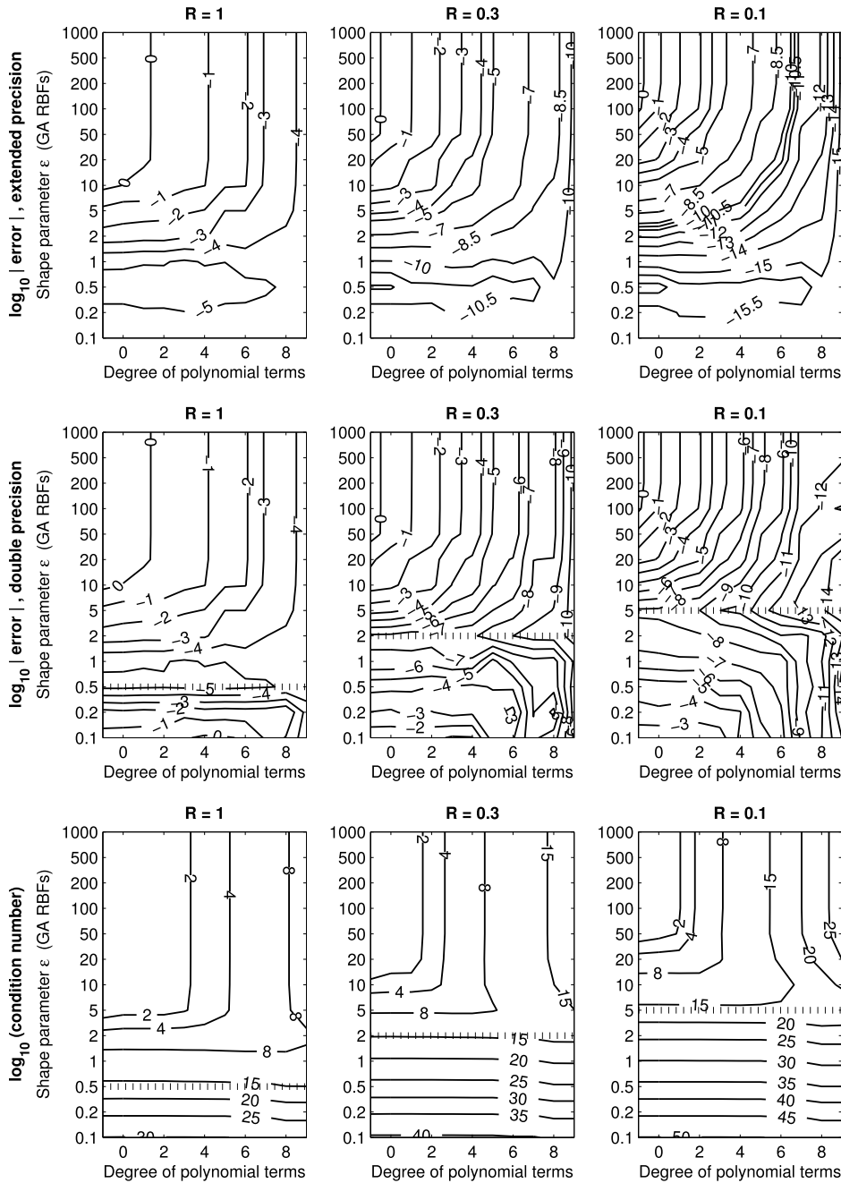
Fig. 6. Top two rows: Accuracy ( \log_{10} error) in GA-based RBF-FD approximations, as functions of shape parameter \varepsilon and degree of included polynomial terms, calculated using 80 decimal digits extended precision vs. in standard 16 digit double precision. Bottom row: \log_{10} of the condition number for the system (8) (calculated using 80 decimal digits extended precision). The level curves utilize interpolation since the polynomial degree can only take on integer values.
