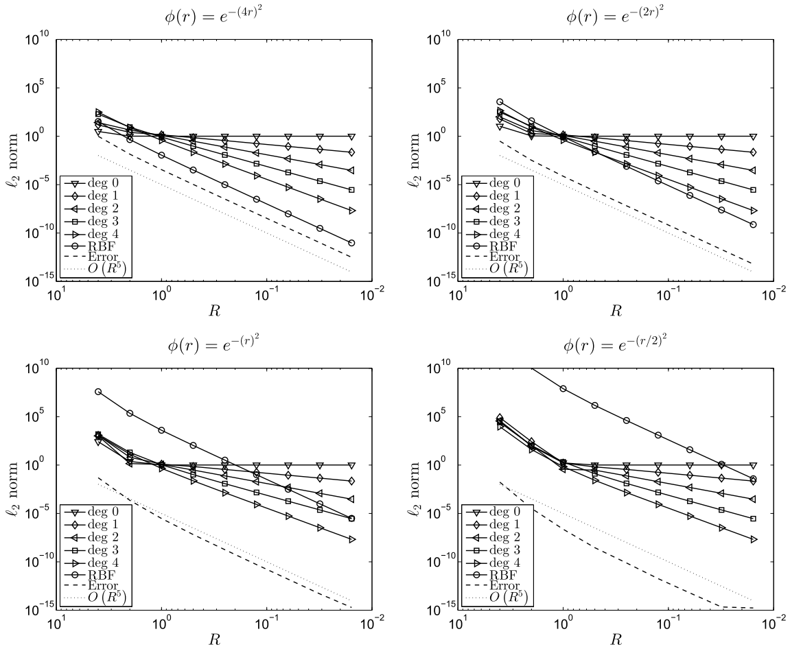
Fig. 9. Behavior of the GA and polynomial coefficients under refinement, where the latter have been separated according to polynomial degree. For the shape parameters 4, 2, 1, and 1/2, the condition numbers of the interpolation matrix are 7 \times 10^2 , 9 \times 10^4 , 2 \times 10^{10} , and 1 \times 10^{16} , respectively. In every case, the RBF coefficients converge to zero at the same rate as the interpolation error.
