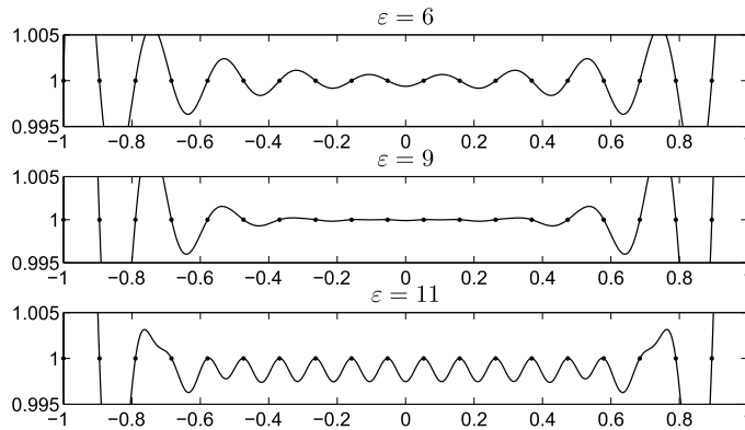
Fig. 2. The GA RBF interpolant for data equal to one on x = [-1, 1] using n = 20 equi-spaced nodes. The top graph displays the interpolant for \varepsilon = 6 , the middle \varepsilon = 9 and the bottom \varepsilon = 11 .
