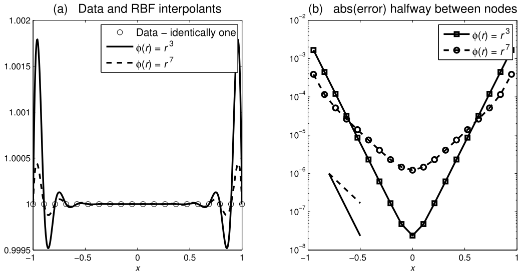
Fig. 10. (a) The RBF interpolants for constant equi-spaced data using n = 20 nodes and PHS \phi(r) = r^3 and \phi(r) = r^7 . (b) The errors at the half-way points between the nodes, corresponding roughly to the extrema of the oscillations in the interpolants. The errors decrease towards the interval center closely following the theoretical rates (16) for the two corresponding spline cases, shown by the short straight line segments at the bottom left.
