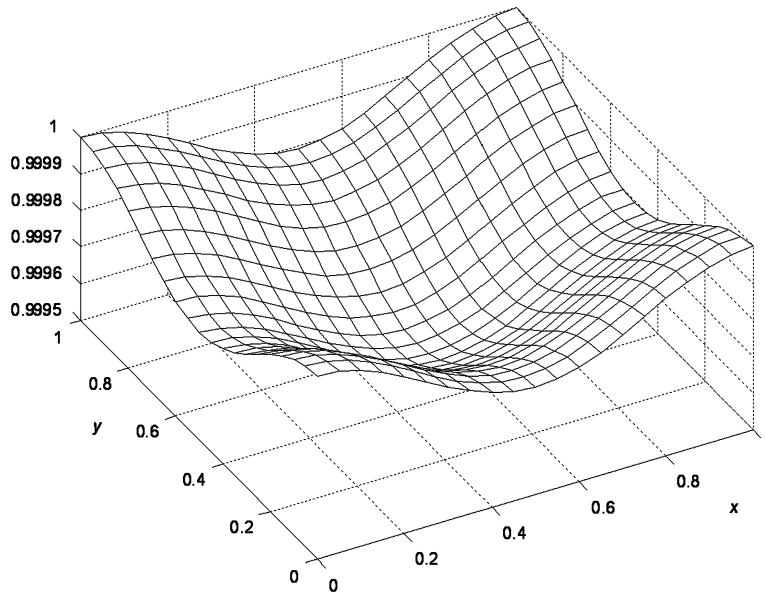
Fig. 1. The GA interpolant to node data that is identically one on an infinite 2-D unit spaced lattice, shown in the case of \varepsilon = 1/h , with h = 1 , over its period [0, 1] \times [0, 1] .
