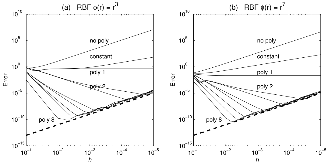
Fig. 11. The worst error encountered when approximating the Laplacian of (12) using the n = 56 node PHS-based RBF-FD stencils, as described in the text. The curve legends ('no poly', 'constant', etc.) are in exactly the same locations in the two subplots, illustrating that the change when going from \phi(r) = r^3 to \phi(r) = r^7 indeed is minimal. The slopes of the different curves perfectly match the predictions (including the thick dashed lines, which mark \text{Error} = 10^{-15}/h^2 ).
