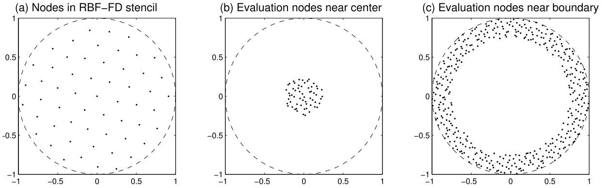
Fig. 4. (a) RBF-FD stencil ( n = 56 nodes) in the case of R = 1 . Parts (b) and (c): Two sets of evaluation points at which the approximation's interpolation accuracy is evaluated.
