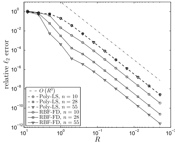
Fig. 14. Convergence comparison for approximation of the test function in (12). In all cases, polynomials up to degree two are included, and in the RBF-FD cases PHS \phi(r) = r^5 are used. Note that increasing the stencil size has no effect on the polynomial least squares error (the three least-square error curves are indistinguishable in the figure). Including RBFs with the polynomials does not change the rate of convergence, but greatly improves the error for each value of R as the stencil is increased, consistent with the low polynomial degree curves in Fig. 12.
