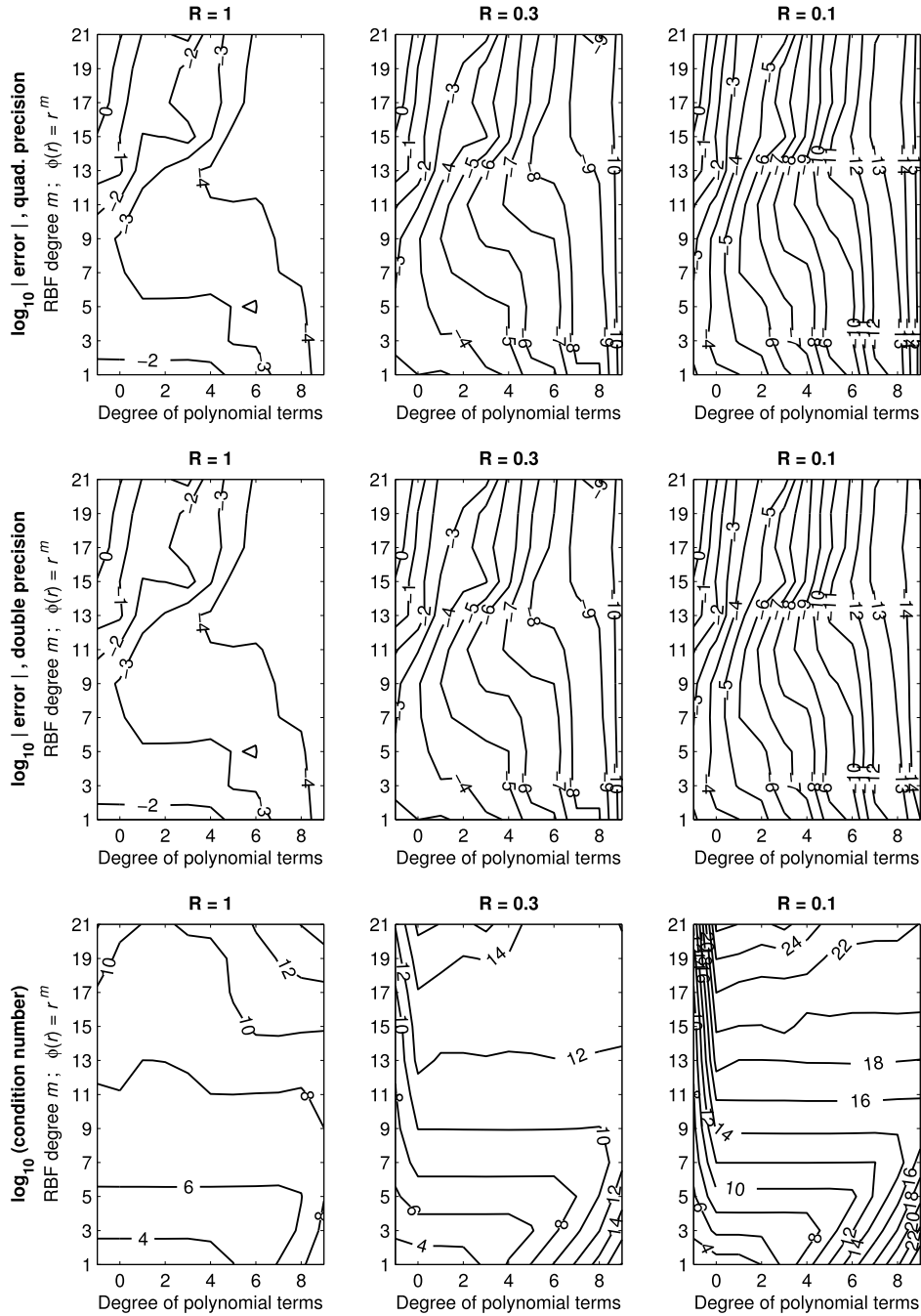
Fig. 7. Top two rows: Accuracy ( \log_{10} error) in PHS-based RBF-FD approximations, as functions of the RBF degree and the degree of included polynomial terms, calculated using 34 decimal digits quad precision vs. in standard 16 digit double precision, Bottom row: \log_{10} of the condition number for the system (8) (calculated using quad precision). As in Fig. 5, plotting the level curves utilizes interpolation as 1) the polynomial degree can only take on integer values and 2) the RBF degrees m are odd integers.
