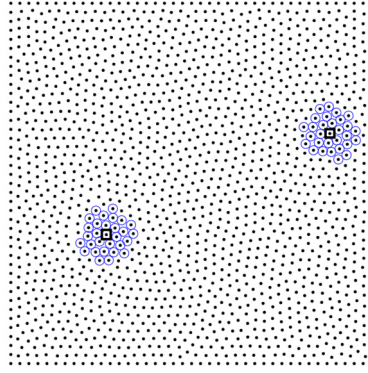
Fig. 3. Illustration of two different RBF-FD stencils in a square domain.
