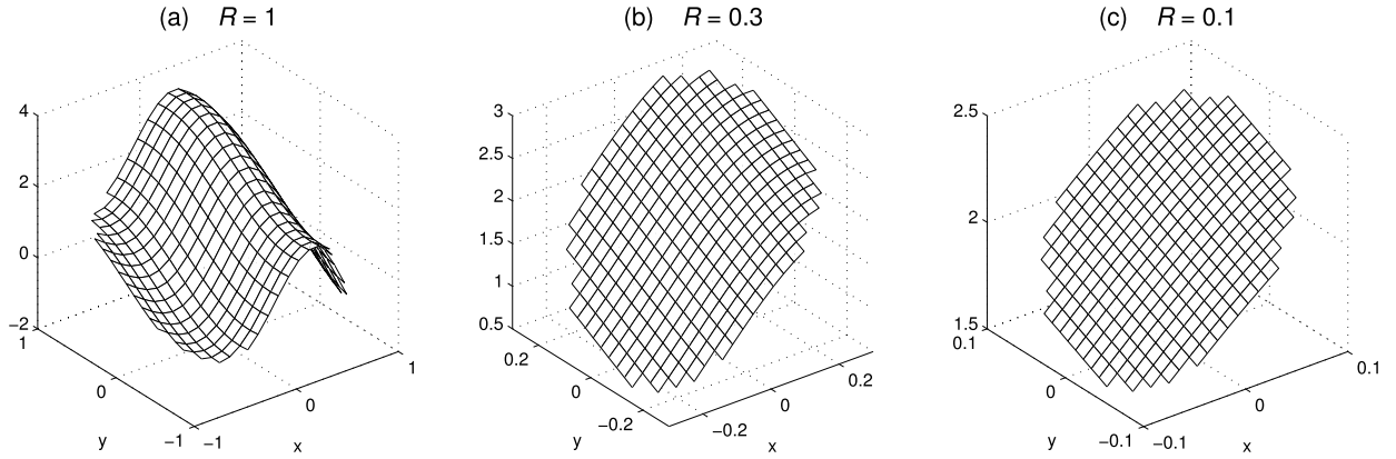
Fig. 5. Test function (12), when displayed over x^2 + y^2 \leq R^2 , with R = 1 , R = 0.3 , and R = 0.1 , respectively.
