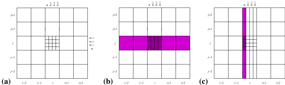
Fig. 3. (a) The twenty-five coarse cells in 2D used to interpolate the sixteen fine-cell averages in cell i for a uniform refinement of R = 4 . (b) The cells involved in the partial interpolation in the x -direction for cell i . The result are the four cell averages that are fine in the x -direction but coarse in the y -direction. (c) The cells involved in the partial interpolation in the y -direction for sub-cells at fine-grid location Ri . This is repeated for all fine-grid locations in the x -direction.
