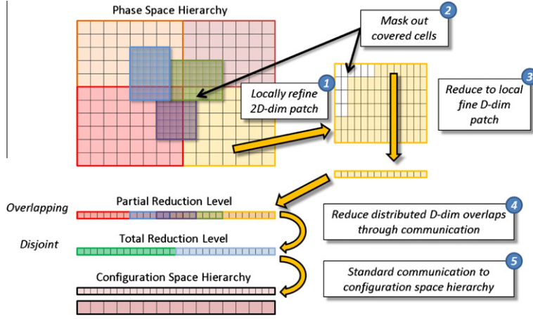
Fig. 5. Graphical depiction of the Mask Reduction Algorithm.
