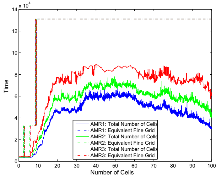
Fig. 10. Time history of the number of cells for the bump-on-tail simulation for the three AMR parameter configurations. The dashed curves are the number of cells in an equivalent uniform grid based on the current maximum refinement level, while the solid curves are the actual number of cells in the AMR hierarchy. Note that around t = 3, 6 and 9 , there is some intermittency in all cases, as the adaptivity adds and removes a small number of patches at the next finer level.
