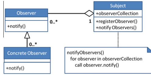
Fig. 8. Unified Modeling Language depiction of the Observer Design Pattern used to create notifying hierarchies. In our case, the reduction and injection algorithms for configuration-space are HierarchyObservers . These observers register themselves with the phase space NotifyingHierarchy to receive notices about regridding.
