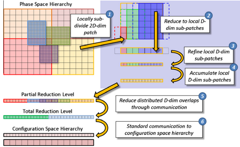
Fig. 6. Graphical depiction of the Sub-Patch Reduction Algorithm. It is those steps in the light purple box that differ from the Mask Reduction Algorithm.
