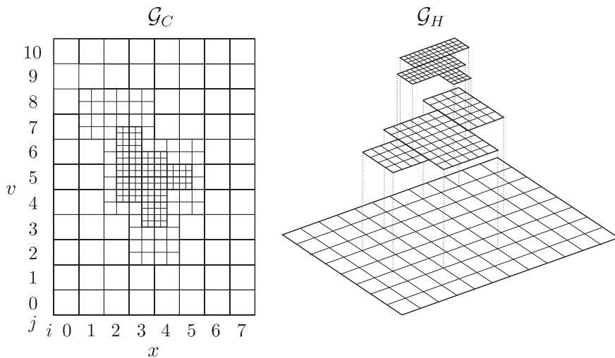
Fig. 1. An example of a three-level, block-structured AMR hierarchy. On the left, the composite refined grid \mathcal{G}_C is shown. On the right, the corresponding mesh hierarchy \mathcal{G}_H with overlapping patches is shown. All patches on the same level have the same refinement ratio relative to the coarsest level; in this case, the refinement ratios are two and four for the intermediate and finest levels, respectively. Note that each level is comprised of a collection of patches completely contained within the patches of the next coarser level.
