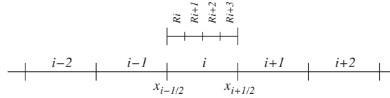
Fig. 2. Relationship of fine to coarse mesh in global index space with a refinement ratio of R = 4 . The five coarse cells shown are used to determine the cell averages in the four fine cells that subdivided cell i .
