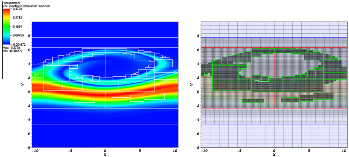
Fig. 9. Example result for the bump-on-tail problem at time t = 22.5 for the AMR1 case. On the left, the distribution function is shown. Boxes outlined in white denote AMR patches. On the right, the corresponding four-level AMR mesh is shown. The mesh adapts to resolve the particle trapping region as it forms. Note that the minimum distribution function is small but negative; no positivity enforcement schemes were used in this calculation.
