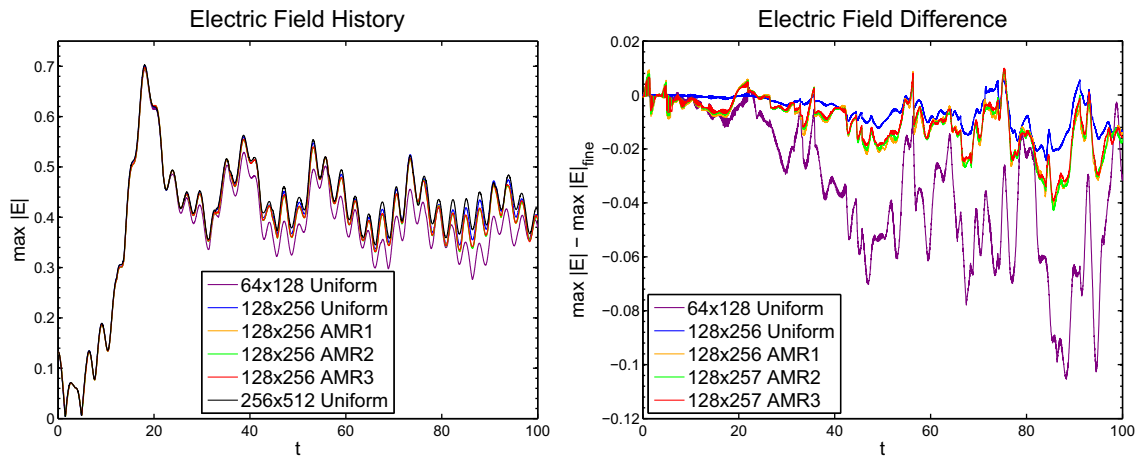
Fig. 11. Time history of the maximum electric field for bump-on-tail calculations at several resolutions. Results are from the three AMR configurations in which the finest resolution is equivalent to a 128 \times 256 uniform mesh as well as reference uniform-grid calculations on meshes of 64 \times 128 , 128 \times 256 , and 256 \times 512 . The left plot shows the maximum of the electric field. The right plot is the same data, plotted as the difference from the results from the fine 256 \times 512 mesh.
