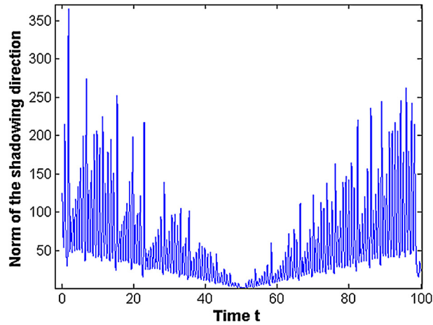
Fig. 2. Norm of \check{v}_{\check{t}} with respect to t for \rho = 28 .
