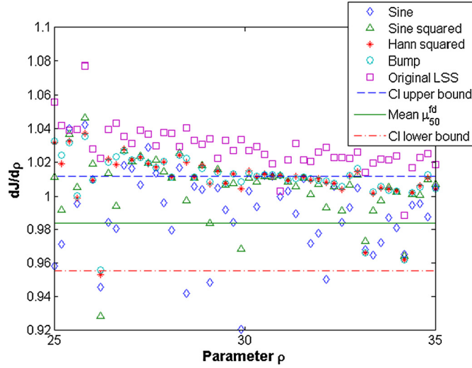
Fig. 3. \frac{d(z)}{d\rho} using different windowing functions and original LSS for integration time T = 50 .
