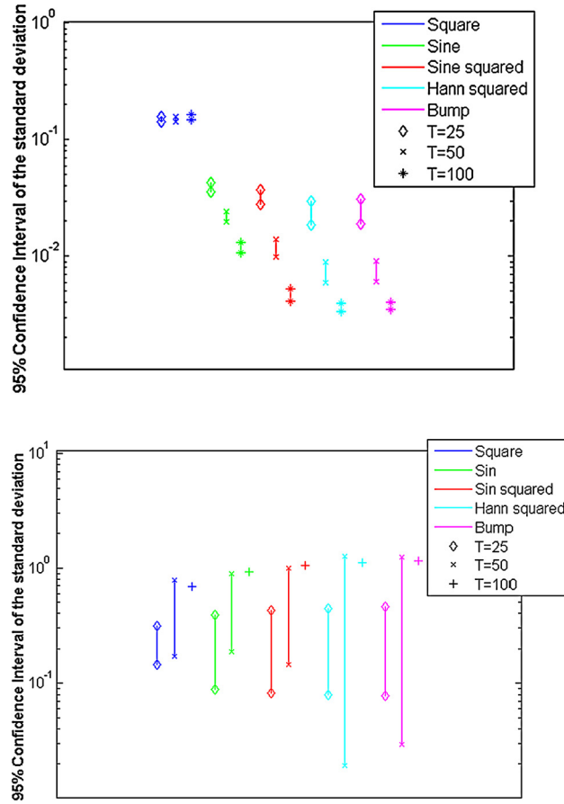
Fig. 4. Standard deviation confidence intervals for \rho = 28 (upper graph) and \rho = 50 (lower graph) using different windowing functions.
