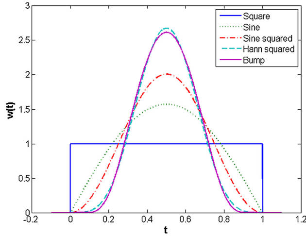
Fig. 1. Shape of the different windowing functions.
