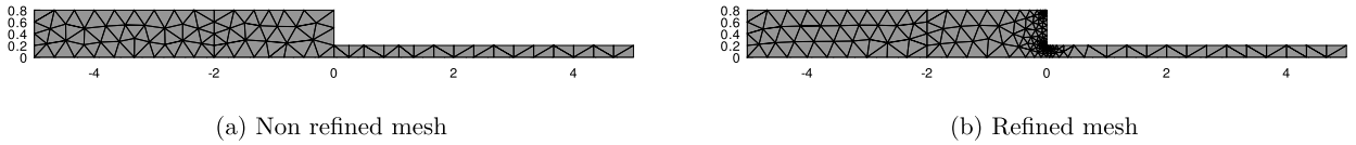
Fig. 4. The two meshes used for the junction of waveguides case-test.
