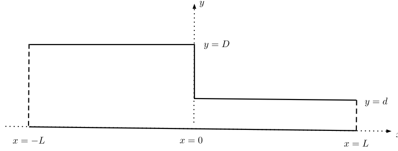
Fig. 3. Schematic view of the junction of the waveguides
