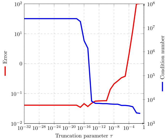
Fig. 1. Parameter \tau versus the error in % and an estimate of the condition number of the final linear system to be solved. (For interpretation of the colors in the figure(s), the reader is referred to the web version of this article.)
