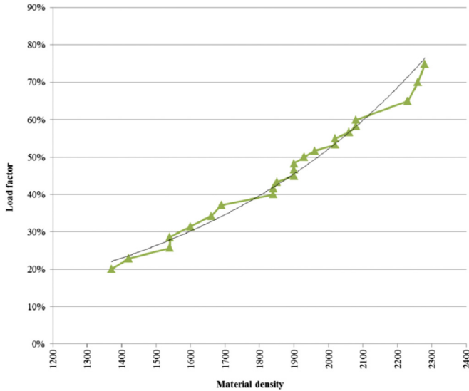
Fig. 3. Relationship between load factor and material density.
