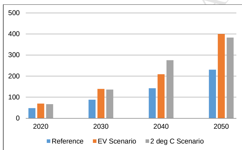
Fig. 4. Electricity demand in transport (TWh)
