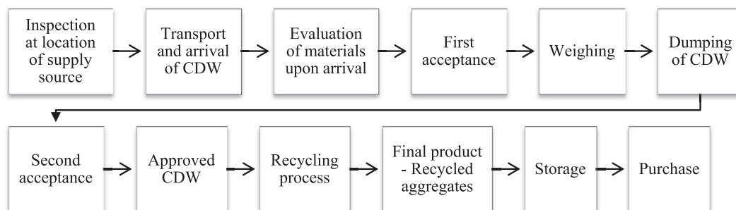
Fig. 6. Proper procedure for acceptance and processing of CDW at recycling plants (adapted from Hendriks, 1998).
