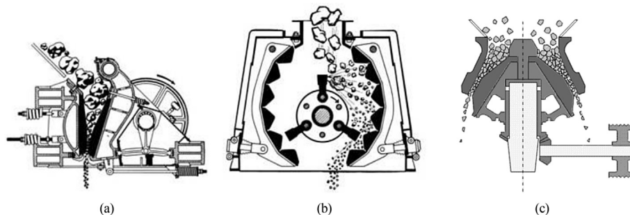
Fig. 8. Examples of (a) a jaw crusher (b) an impact crusher and (c) a cone crusher (Crushersale, 2013; Penncrusher, 2013).
