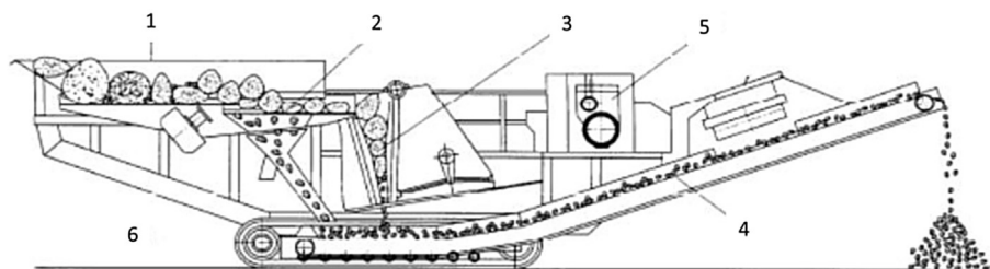
Fig. 5. Example of a mobile crusher (1 - feeding hopper; 2 - oscillating conveyor; 3 - jaw crusher; 4 - discharging transport belt; 5 - diesel engine as power unit; 6 - mobile by wheels, crawlers or skids) (adapted from Kumbhar et al. (2013)).
