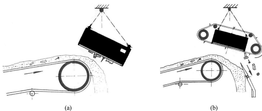
Fig. 9. Fixed electromagnets (a) and rotating magnetic belts (b) (adapted from Nordberg (1994)).
