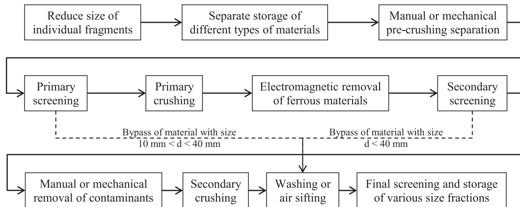
Fig. 7. Recycling procedure of CDW (adapted from Hansen (1992)).
