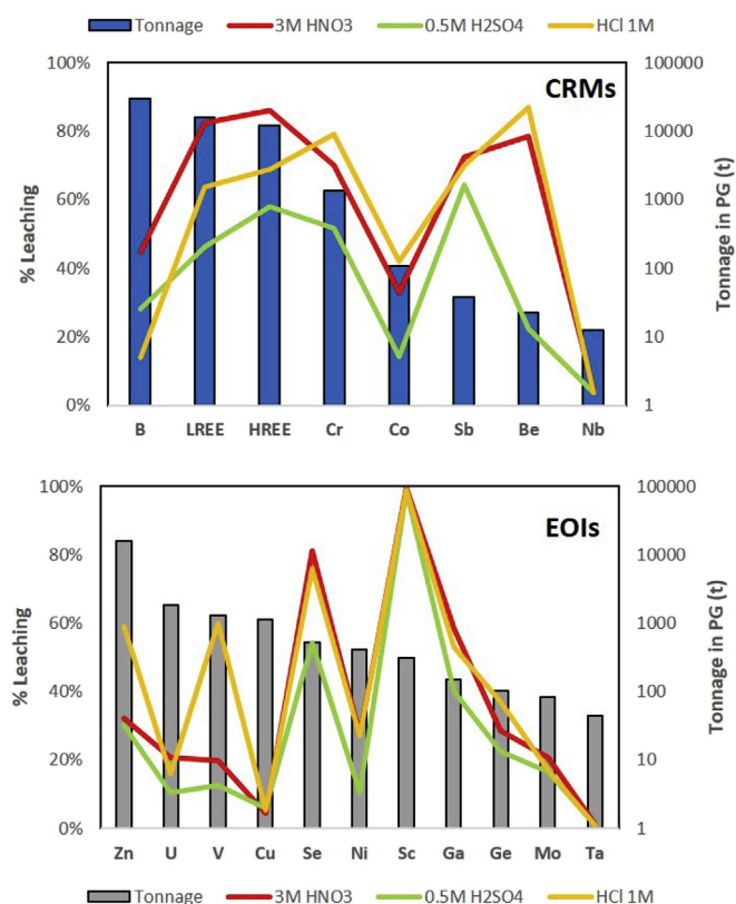
Fig. 4. Leaching rates of some elements of economic interest from PG using different acid solutions (i.e. 0.5 M \text{H}_2\text{SO}_4 , 1 M HCl and 3 M \text{HNO}_3 ).
