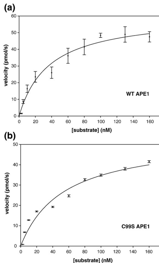
Fig. 5. Reaction kinetics of WT and C99S mutant APE1 (33 pM) in the presence of 2 mM [Mg^{2+}] . (a) WT APE1 and (b) C99S mutant proteins were incubated with 0–160 nM of THF-containing oligonucleotide at 37 °C for 3 min. Other details are described in Materials and Methods. Data represent mean values of four independent experiments.
