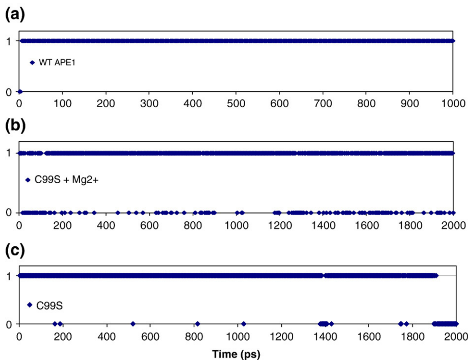
Fig. 6. Kinetics of H-bond formation/breakage between NE2 of H309 and O1P of the AP-site phosphate for (a) WT APE1, (b) C99S mutant with Mg^{2+} at the B site, and (c) C99S APE1 mutant. The value is 1 when a H bond is formed and 0 when not formed.
