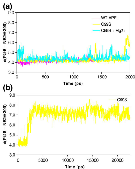
Fig. 7. Time course of the distance between atoms NE2 on the His309 and P on the AP site for (a) WT APE1, C99S and C99S+ Mg^{2+} simulations and (b) C99S APE1 mutant simulation.
