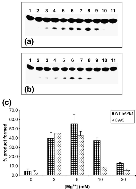
Fig. 4. Effect of Mg^{2+} on AP-endonuclease activity of (a) WT and (b) C99S mutant APE1. Lane 1, control; lanes 2–11, 0, 0.1, 0.5, 1, 2, 3, 5, 10, 20, and 40 mM Mg^{2+} , respectively. Lane 2 also contains 0.1 mM EDTA. (c) Effect of Mg^{2+} on the activity of WT and Ser99 mutants.
