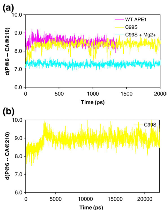
Fig. 8. Typical time course for the distance between atoms CA of Asp210 and P of the AP site for (a) WT APE1, C99S and C99S+Mg 2+ simulations and (b) C99S APE1 mutant simulation.
