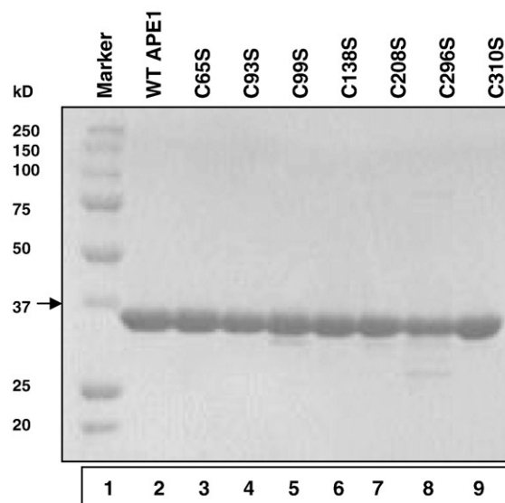
Fig. 1. Purification of WT and mutant (Cys→Ser) APE1 proteins. Coomassie Blue staining of purified WT APE1 and Ser mutants (0.5 \mu g protein) after SDS-PAGE (10% polyacrylamide). Lane 1, protein marker; lane 2, WT APE1; lane 3, C65S; lane 4, C93S; lane 5, C99S; lane 6, C138S; lane 7, C208S; lane 8, C296S; and lane 9, C310S.
