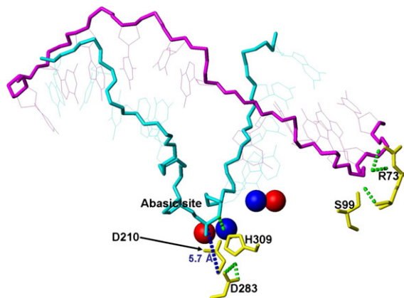
Fig. 10. Snapshots of simulation of the C99S mutant after 500 ps with two Mg^{2+} ions in the active site. The positions of key DNA residues and Mg^{2+} are shown. The final Mg^{2+} positions are shown in red; for comparison the starting positions, which are identical to the unperturbed precleavage A and B site, are shown in blue. Important H bonds are shown as dotted green lines.
