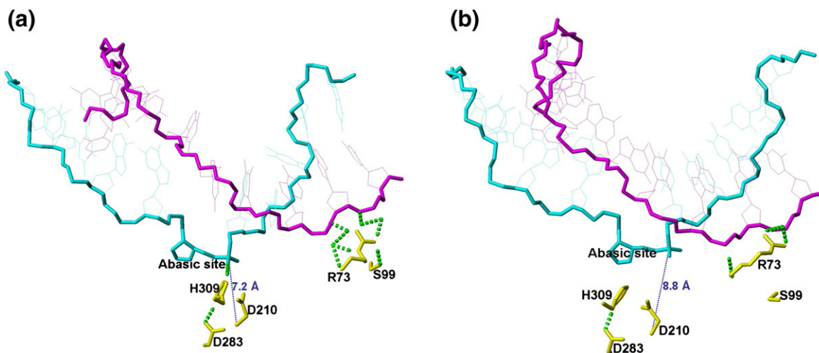
Fig. 9. Snapshots of the C99S mutant simulation at the beginning after 1 ps (a) and at the end after 22,500 ps (b). Only the DNA and key residues that are important for this study in the C99S mutant protein are shown. The AP-site-containing DNA strand is shown in cyan and the complementary strand in magenta. The side chains of key residues of the C99S mutant are shown in yellow. Dotted green and blue lines represent H bonds and the distance is indicated.
