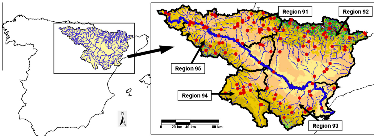
Fig. 1. Location of the Ebro River catchment. Solid points show location of the gauging stations used in the study.
