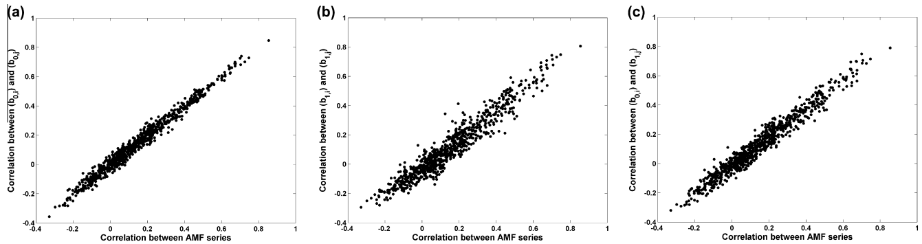
Fig. 3. Correlation between AMF series and PWMs. (a) Between first-order PWMs ( b_0 ); (b) between second-order PWMs ( b_1 ); and (c) between first-order and second-order PWMs ( b_0 and b_1 ).
