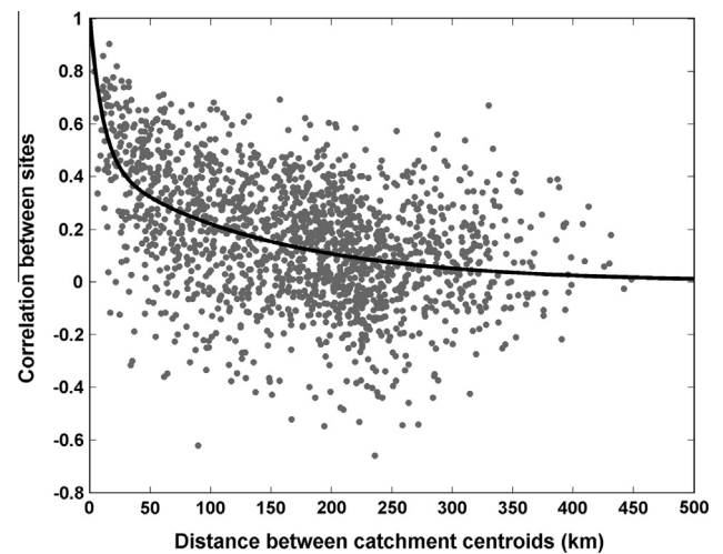
Fig. 4. Correlation between AMF series and distance between catchment centroids for the 93 flood series from the Ebro catchment. Solid line shows the double exponential function fitted using the least square technique.
