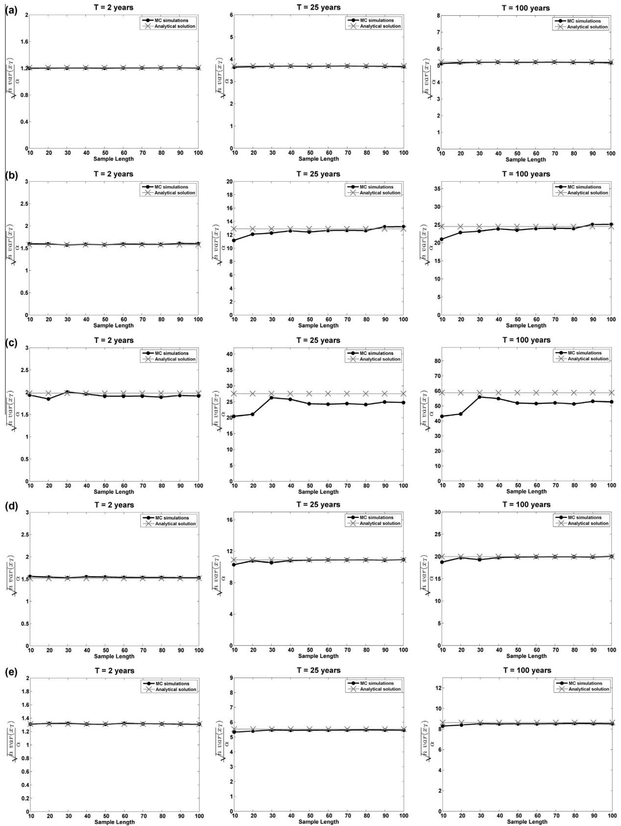
Fig. 2. Comparison between sampling variance estimated by Monte Carlo simulations and the analytical solution estimated by Taylor series approximation. Regions by rows: (a) Region 91; (b) Region 92; (c) Region 93; (d) Region 94; and (e) Region 95. Return period by columns.
