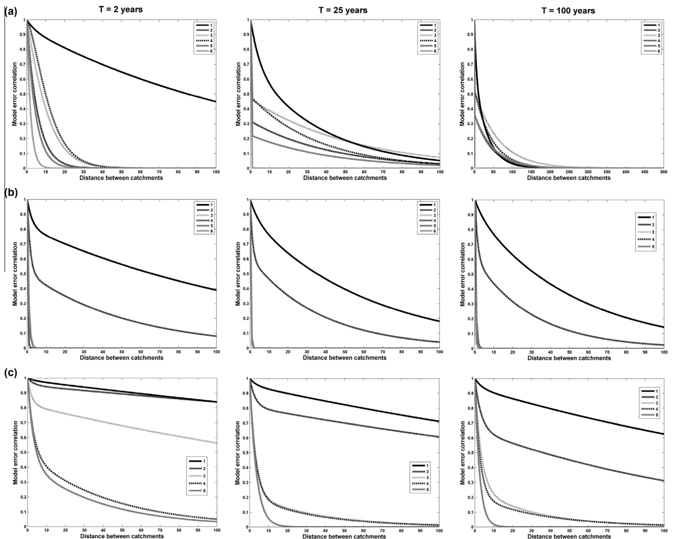
Fig. 6. Evolution of correlation of residuals with distance between sites in \text{km}^2 . Regions by rows: (a) Region 91; (b) Region 92; and (c) Entire Ebro River catchment. Return period by columns.
