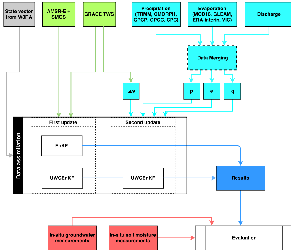
Figure 2: A schematic illustration of the UWCEKF steps applied for data assimilation, as well as data merging process.
