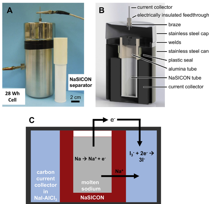
Fig. 3. (A) Photograph of prototype 28 Wh (10 Ah) NaI battery assembly with NaSICON separator at right. (B) 3D model of the 28 Wh NaI battery assembly. (C) Schematic of battery (not to scale) depicting chemical reactions and ion movement upon battery discharge.
