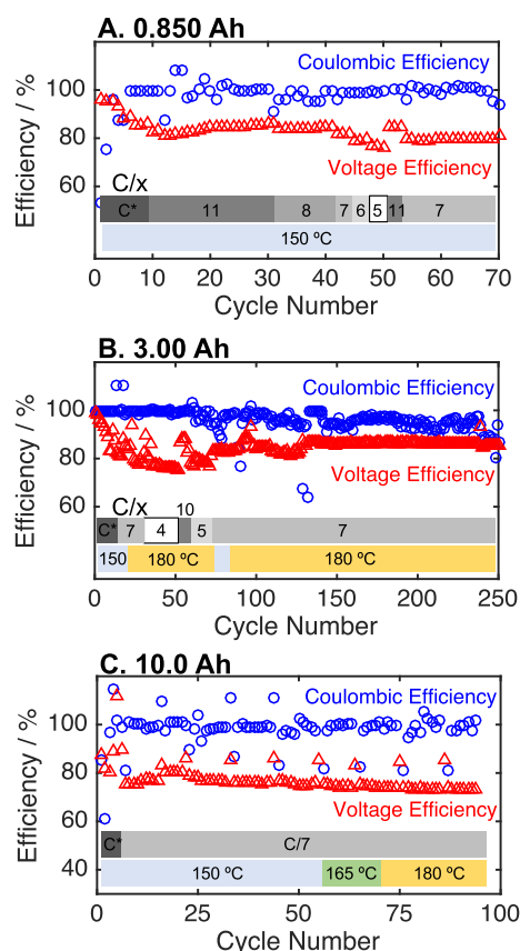
Fig. 4. Coulombic efficiency, voltage efficiency, operating temperature, and discharge rate for NaI batteries of different sizes (A) 0.850 Ah, (B) 3.00 Ah, (C) 10.0 Ah. For (C) every 11th cycle is at C/15. "C" indicates a series of initial conditioning steps at low rates.
