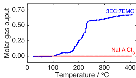
Fig. 6. Molar gas output (moles of gas produced per moles of electrolyte) for the NaI-AlCl 3 electrolyte of the NaI battery compared to a standard Li-ion electrolyte, 1.2 M LiPF 6 in EC:EMC (3:7).
