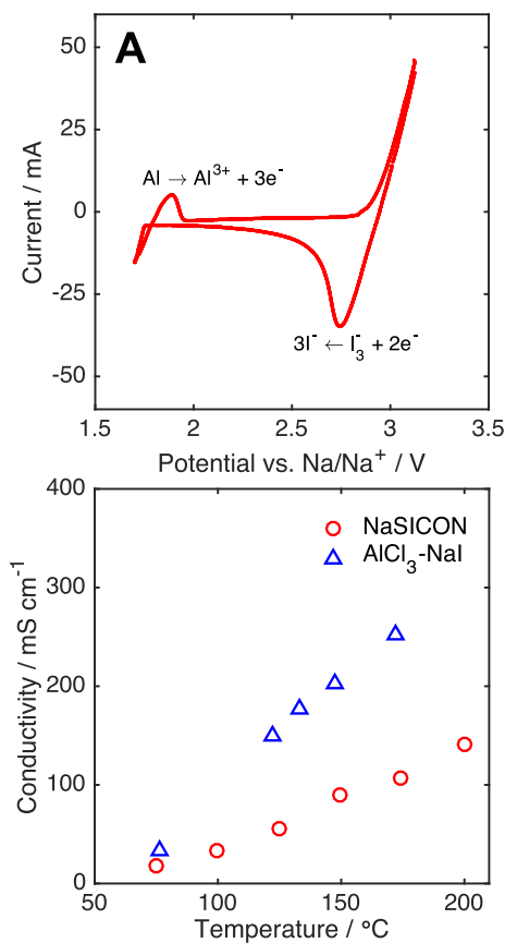
Fig. 2. (A) CV of a carbon felt electrode in the \text{AlCl}_3\text{:NaI} (40:60 at%) catholyte at 125 ^\circ\text{C} and 100 \text{mV s}^{-1} . (B) Ionic conductivity of the \text{AlCl}_3\text{:NaI} catholyte and Ceramtec NaSICON as a function of temperature.
