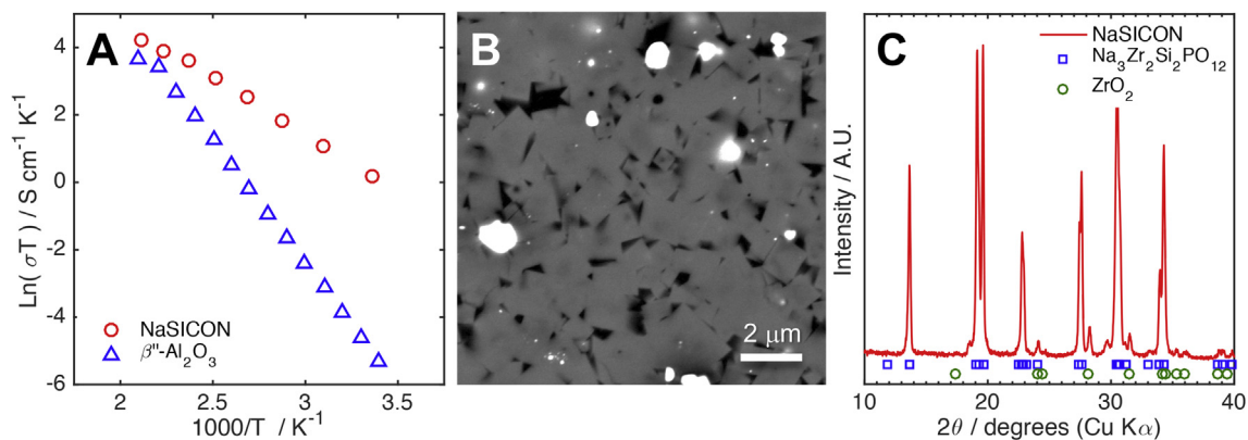
Fig. 1. Characterization of the NaSICON separator: (A) Arrhenius plot of \text{Na}^+ conductivity vs. inverse temperature for Ceramtec NaSICON compared to that of \beta''\text{-Al}_2\text{O}_3 . (B) Highly-contrasted backscatter SEM micrograph of a polished NaSICON cross section. (C) X-ray diffraction (Cu K \alpha radiation) patterns for Ceramtec NaSICON compared to peak positions for \text{Na}_3\text{Zr}_2\text{Si}_2\text{PO}_{12} and \text{ZrO}_2 (PDF# 04-008-8579 and 01-083-0943).
