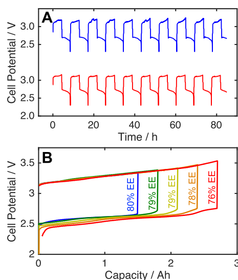
Fig. 5. (A) 3 Ah cell voltage profiles at C/7, 180 °C before (upper, blue) and after (lower, red) idling for 1 week at room temperature. (B) Influence of depth of discharge on the charge-discharge curves and EE of the 3 Ah cell at 150 °C and C/7. (For interpretation of the references to colour in this figure legend, the reader is referred to the web version of this article.)
