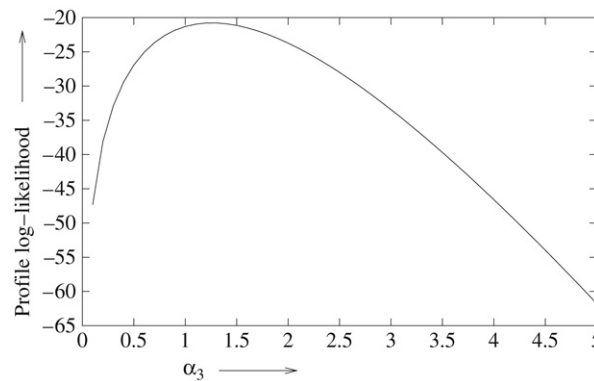
Fig. 1. Profile log-likelihood function of \alpha_3 .
