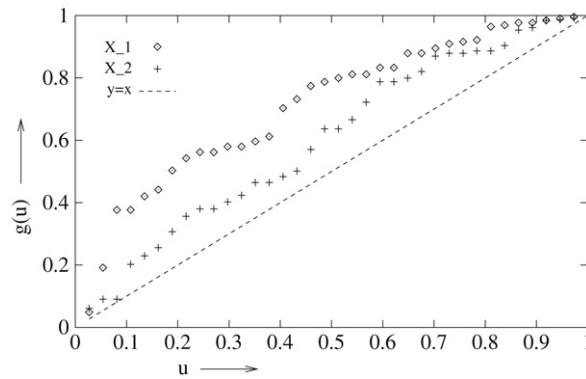
Fig. 2. Scaled TTT transform for X_1 and X_2 .
