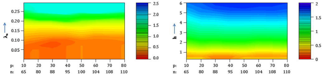
Fig. 3. Colored contours of \|\hat{\beta} - \beta\|_1 on p vs. \lambda_n (left) and h .(right). (For interpretation of the references to color in this figure legend, the reader is referred to the web version of this article.)
