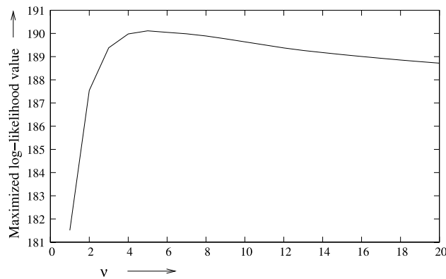
Fig. 3. The maximized log-likelihood value as a profile function of \nu = 1(1)20 .
