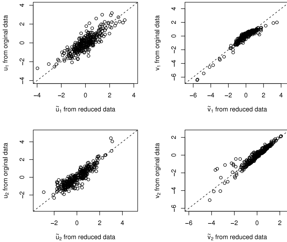
Fig. 1. Scatterplots of the canonical covariates from the original data versus the canonical covariate from the reduced data.
