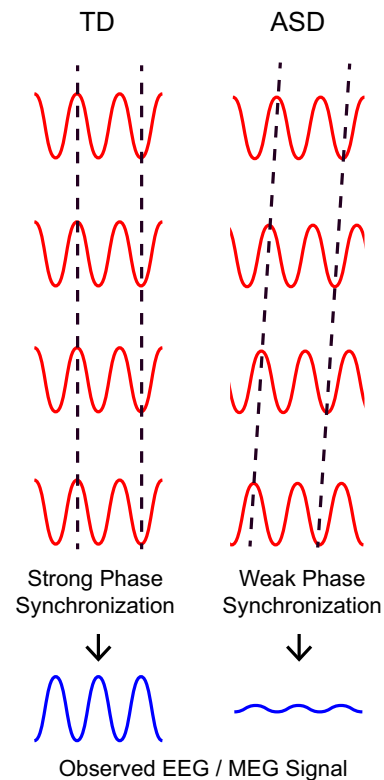
Fig. 2. Reduced oscillatory power as a signature of reduced neural synchronization. Rhythmic shifts in single neuron membrane potentials (top, red) can occur in or out of phase synchronization. TD individuals (left) recruit neural networks with a high degree of phase synchronization, while individuals with ASD (right) have reduced phase synchronization. EEG/MEG signal amplitude diminishes with decreased phase synchronization despite the number of participating neurons and membrane fluctuations being of equal size. (For interpretation of the references to color in this figure legend, the reader is referred to the web version of this article.)
