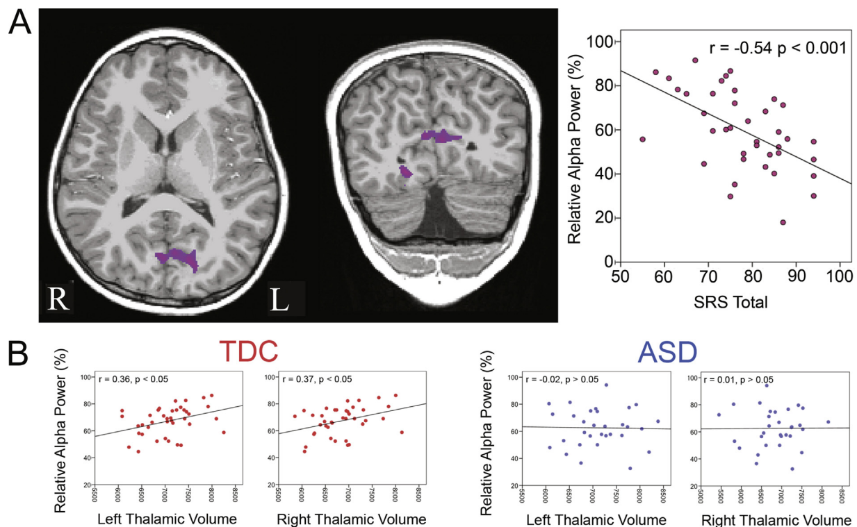
Fig. 7. Thalamocortical connectivity fails to correlate with oscillatory power in ASD. (A) Calcarine sulcus region of interest (ROI; left) & correlation between relative alpha power within this ROI and social responsiveness scale (SRS) total score (right). Lower alpha power is associated with a higher (worse) SRS score. (B) Correlation between thalamic volume and alpha power. Thalamic volume is positively correlated with relative alpha power in typically developing children (TDC) (left), but does not correlate in children with ASD (right). Modified with permission from: James Edgar et al., J. Autism Dev. Disord. , 2015, 45(3):795–804.
