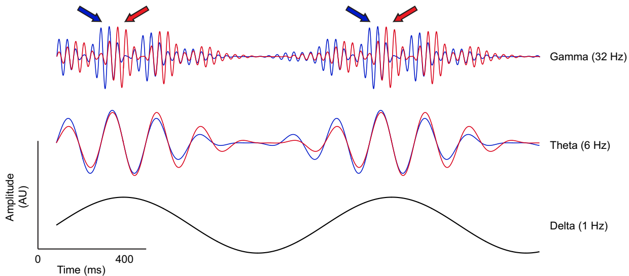
Fig. 4. Disrupted oscillatory hierarchy. Disruption in phase-amplitude coupling between oscillatory frequencies leads to decreased neural synchronization at high frequencies. In this conceptual figure, the red and blue signals indicate theta oscillations in separate neural networks. Coupling for each signal to delta activity is out of phase alignment by 0.25 rad ( 14.3^\circ ). Gamma to theta phase-amplitude coupling is similarly perturbed by 1 rad ( 57.2^\circ ). Despite identical gamma phase between the two signals, gamma power is highly misaligned, resulting in desynchronization of periods where neural firing will be maximal (red and blue arrows). A very low gamma frequency (32 Hz) and large phase offsets (0.25 & 1 rad) are used here for ease of visualization. (For interpretation of the references to color in this figure legend, the reader is referred to the web version of this article.)
