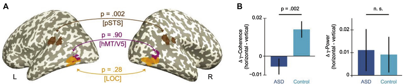
Fig. 5. Reduced interhemispheric gamma coherence in ASD during slit viewing of objects. Recognition of objects passing behind a moving slit requires integration across visual hemi-fields when the slit is horizontal, but does not require integration when the slit is vertical. (A) Brain regions demonstrating reduced interhemispheric gamma synchronization in ASD during horizontal slit viewing of visual objects. (pSTS = posterior superior temporal sulcus, hMT/V5 = human motion area, LOC = lateral occipital area). The p values indicate the significance for the group (typically developing or ASD) \times condition (vertical slit vs horizontal slit) interaction for interhemispheric gamma synchronization. (B) Interhemispheric synchronization between the two posterior superior temporal sulci is enhanced during horizontal slit viewing in typically developing individuals, but not for individuals with ASD. Local synchronization (power) is unaffected. Reproduced with permission from: Ina Peiker et al., J. Neurosci. , 2015;35:16352–16361.
