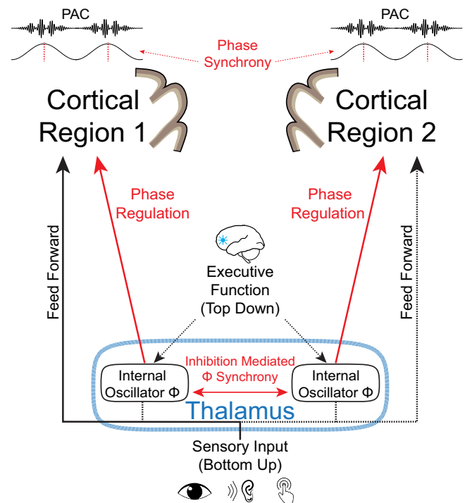
Fig. 6. Model demonstrating reduced cortical synchronization as a result of impaired thalamic coordination. The internal circuitry of the thalamus generates low frequency coordination signals in response to both top down (executive) and bottom up (sensory) inputs. These low frequency coordination signals then synchronize activity at disparate cortical regions through phase-amplitude coupling. Reduced cortical synchronization in ASD results from impaired coordination between thalamic oscillators and/or impaired regulation of cortical phase by thalamic inhibition. Phase amplitude coupling to desynchronized low frequency oscillation then results in impaired high frequency synchronization between cortical regions.
