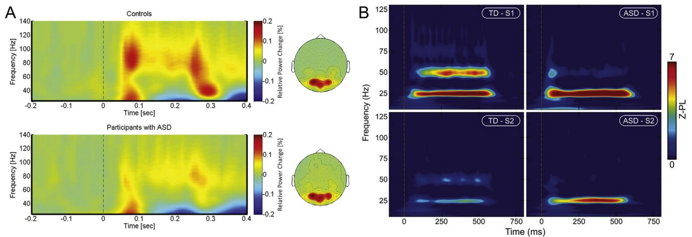
Fig. 3. Gamma synchronization during sensory processing is reduced in ASD. (A) Time frequency representation of neural responses to Mooney faces in typically developing (control) individuals (top) and individuals with ASD (bottom). Topographic representations are averaged for the time interval from 0–400 ms after onset of the stimulus and across frequencies from 25–120 Hz. Note that on the time-frequency plots that induced gamma power is significantly reduced in individuals with ASD. Reproduced with permission from: Limin Sun et al., J. Neurosci. 2012;32:9563–9573. (B) Time frequency representation of neural responses to 25 Hz vibrotactile stimulation in primary somatosensory cortex (S1; top) and secondary somatosensory cortex (S2; bottom) in both TD (left) and ASD (right) individuals. Note that the TD individuals show significantly more 50 Hz phase locking in both S1 and S2 than individuals with ASD. Reproduced with permission from: Sheraz Khan et al., Brain 2015;138:1394–1409. (For interpretation of the references to color in this figure legend, the reader is referred to the web version of this article.)
