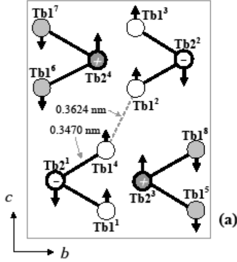
Figure 9. (a) Magnetic structure of Tb 3 Ni 2 Ge 3 below ~33 K and down to 17 K and (b) additional low-temperature magnetic component in the Tb 3 Ni 2 Ge 3 magnetic structure (from 15 K and down to 1.5 K). The shortest Tb1-Tb1 and Tb1-Tb2 interatomic distances are shown in Figure.
