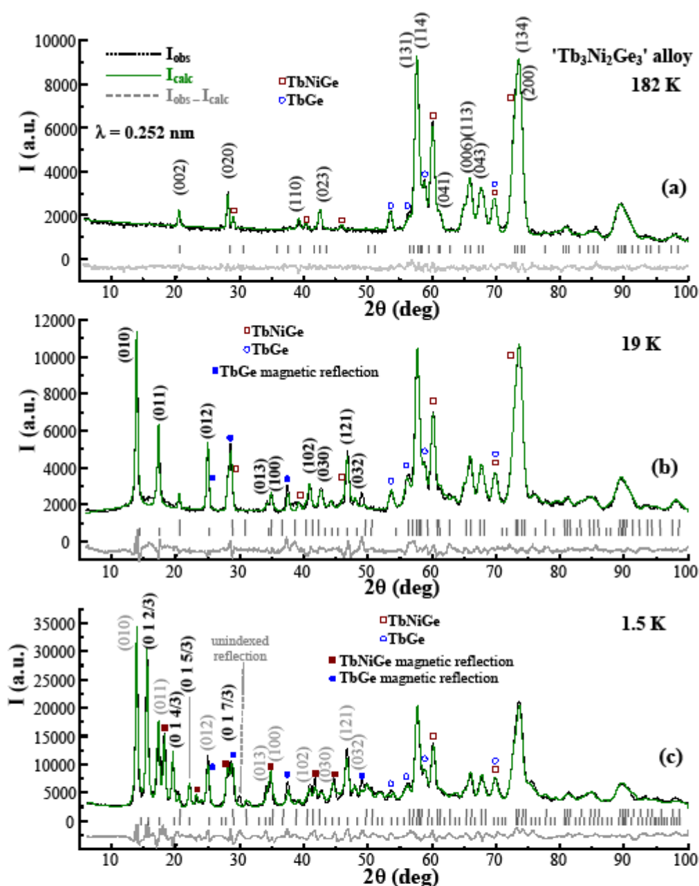
Figure 7. Neutron diffraction patterns of \text{Tb}_3\text{Ni}_2\text{Ge}_3 sample (a) at 182 K (paramagnetic state of \text{Tb}_3\text{Ni}_2\text{Ge}_3 ), (b) at 19 K ( ac -antiferromagnetic ordering of \text{Tb}_3\text{Ni}_2\text{Ge}_3 : (\text{AF}_a + \text{AF}_c)^{\text{K}_0} ( \text{C}2'/c ) with \text{K}_0 = [0, 0, 0] vector and (c) at 1.5 K ( ac -antiferromagnetic ordering of \text{Tb}_3\text{Ni}_2\text{Ge}_3 : (\text{AF}_a + \text{AF}_c)^{\text{K}_0} ( \text{C}2'/c ) + \text{AF}_a^{\text{K}_1} with \text{K}_0 = [0, 0, 0] and \text{K}_1 = [0, 0, \pm 1/3] vectors). The first row of ticks refers to the nuclear Bragg peaks whereas the second row of lines refers to the magnetic reflections of \text{Tb}_3\text{Ni}_2\text{Ge}_3 . The (hkl) indices of the strongest magnetic reflections of \text{Tb}_3\text{Ni}_2\text{Ge}_3 are indicated in Figures 7b and 7c. The strongest structural and magnetic reflections of the \text{TbNiGe} and \text{TbGe} impurities are marked in Figures.
