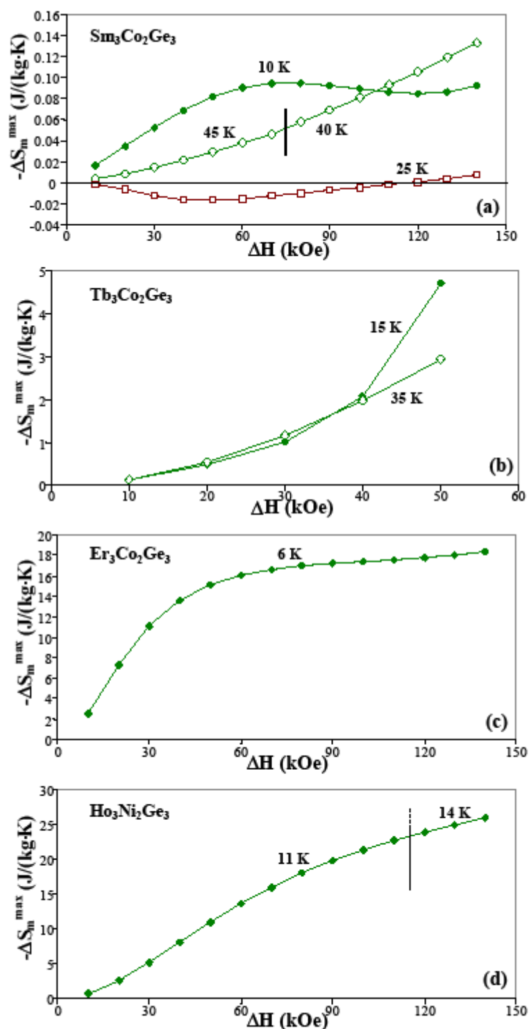
Figure 6. The magnetic entropy change of corresponding magnetic transitions ( -\Delta S_m^{\max} ) vs. field change ( \Delta H ) of (a) \text{Sm}_3\text{Co}_2\text{Ge}_3 , (b) \text{Tb}_3\text{Co}_2\text{Ge}_3 , (c) \text{Er}_3\text{Co}_2\text{Ge}_3 and (d) \text{Ho}_3\text{Ni}_2\text{Ge}_3 .
