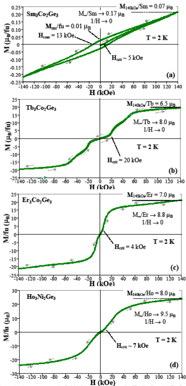
Figure 3. Magnetisation vs. magnetic field of (a) Sm 3 Co 2 Ge 3 , (b) Tb 3 Co 2 Ge 3 , (c) Er 3 Co 2 Ge 3 and (d) Ho 3 Ni 2 Ge 3 at 2 K in fields up to 140 kOe
