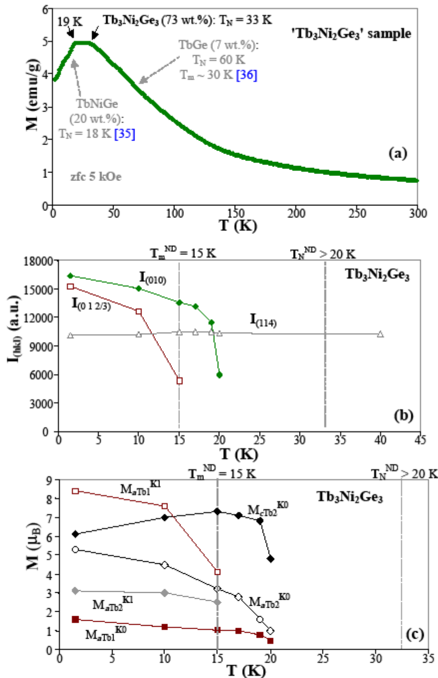
Figure 8. (a) Magnetization as a function of temperature of \text{Tb}_3\text{Ni}_2\text{Ge}_3 sample; (b) thermal evolution of the strongest magnetic reflections I_{(hkl)} in the neutron diffraction patterns of \text{Tb}_3\text{Ni}_2\text{Ge}_3 and (c) M_{\text{Tb1,2}}^{K0} , M_{\text{Tb1,2}}^{K1} the magnetic moments and M_{\text{Tb1,2}}^{K1} , M_{\text{Tb1,2}}^{K0} the amplitude of magnetic moments of Tb1 and Tb2 atoms with the K_0 = [0, 0, 0] and K_1 = [0, 0, \pm 1/3] propagation vectors.
