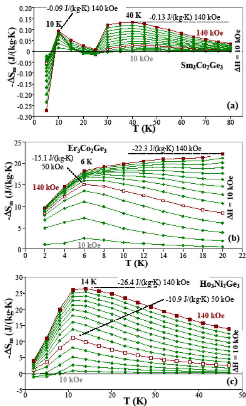
Figure 5. Isothermal magnetic entropy change, -\Delta S_m , of (a) \text{Sm}_3\text{Co}_2\text{Ge}_3 , (b) \text{Er}_3\text{Co}_2\text{Ge}_3 and (c) \text{Ho}_3\text{Ni}_2\text{Ge}_3 for a field change of 0-140 kOe.
