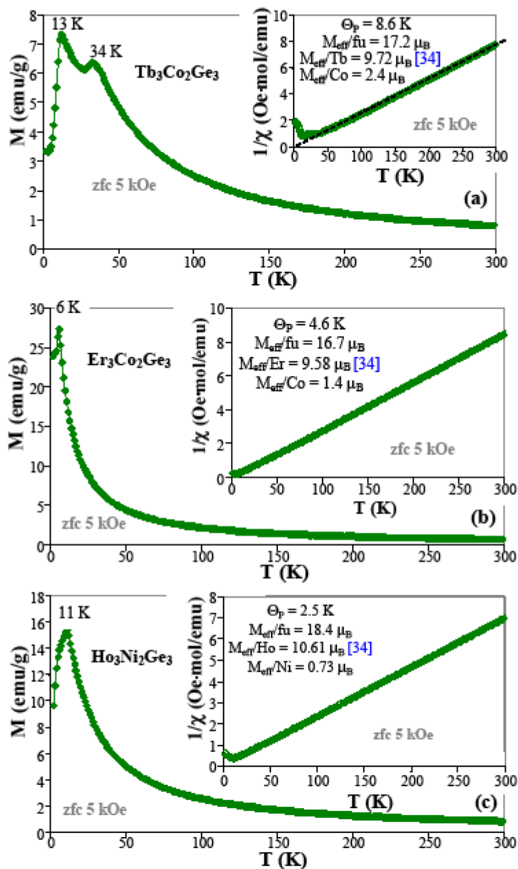
Figure 2. Magnetization as a function of temperature in field of 5 kOe of (a) \text{Tb}_3\text{Co}_2\text{Ge}_3 , (b) \text{Er}_3\text{Co}_2\text{Ge}_3 and (c) \text{Ho}_3\text{Ni}_2\text{Ge}_3 (Insets in Figures: Curie-Weiss fit to the inverse paramagnetic susceptibility).
