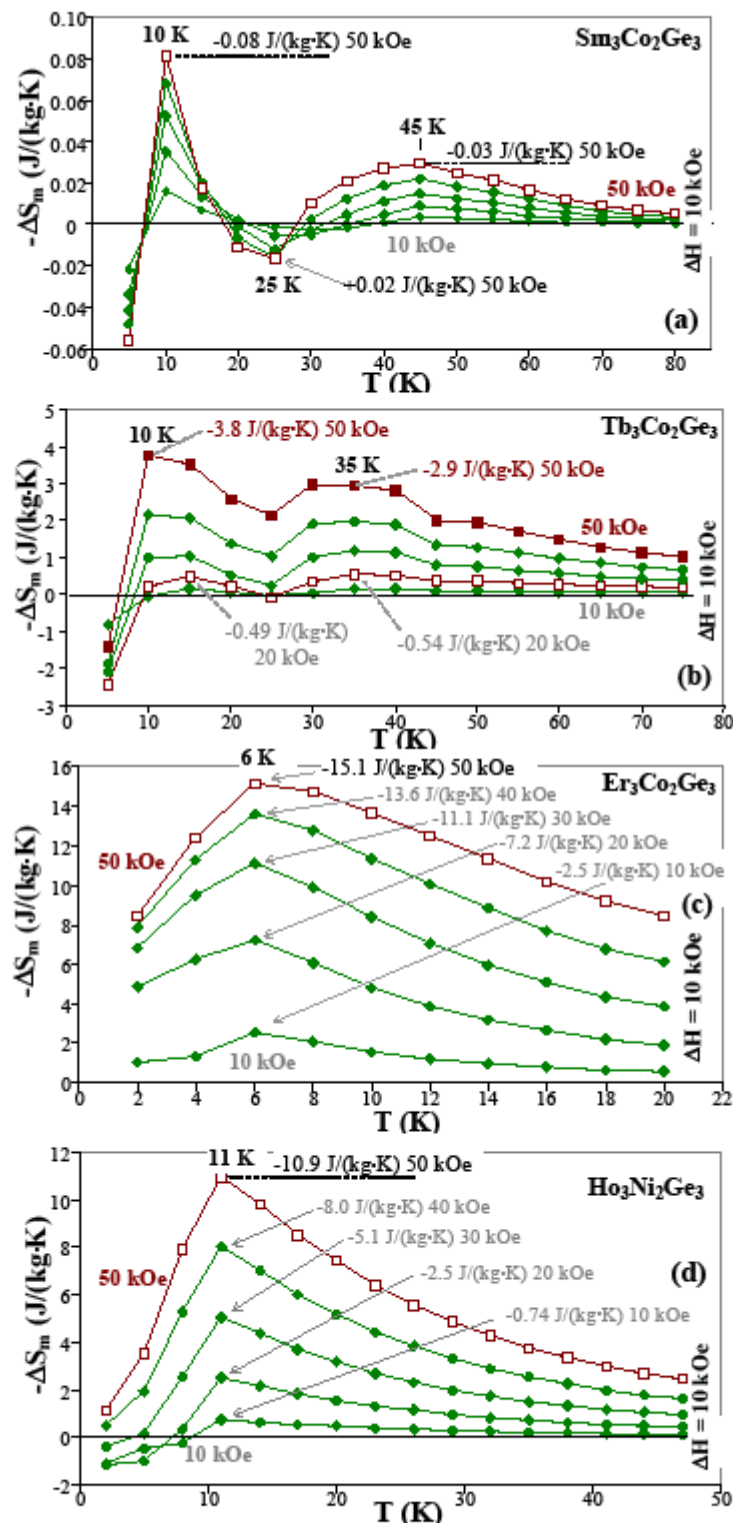
Figure 4. Isothermal magnetic entropy change, -\Delta S_m , of (a) \text{Sm}_3\text{Co}_2\text{Ge}_3 , (b) \text{Tb}_3\text{Co}_2\text{Ge}_3 , (c) \text{Er}_3\text{Co}_2\text{Ge}_3 and (d) \text{Ho}_3\text{Ni}_2\text{Ge}_3 for a field change of 0-50 kOe.
