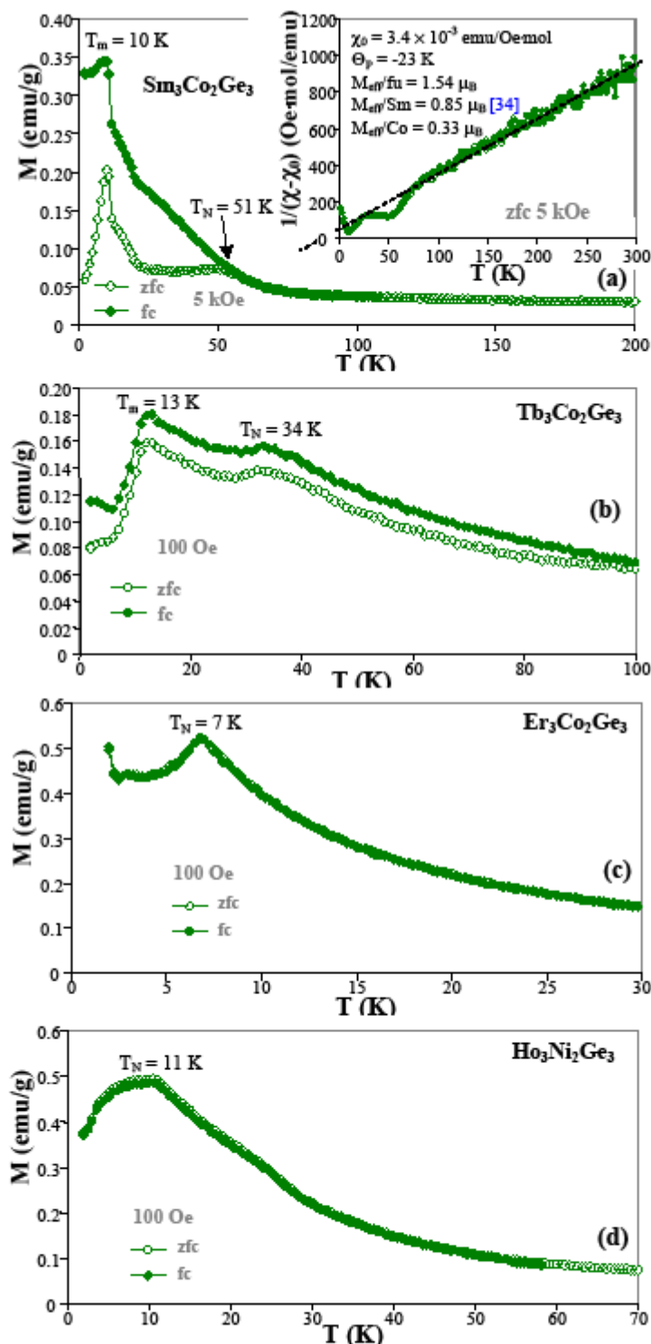
Figure 1. Magnetization as a function of temperature of (a) \text{Sm}_3\text{Co}_2\text{Ge}_3 , (b) \text{Tb}_3\text{Co}_2\text{Ge}_3 , (c) \text{Er}_3\text{Co}_2\text{Ge}_3 and (d) \text{Ho}_3\text{Ni}_2\text{Ge}_3 (Insets in Figure 1a: modified Curie-Weiss fit to the inverse paramagnetic susceptibility).
