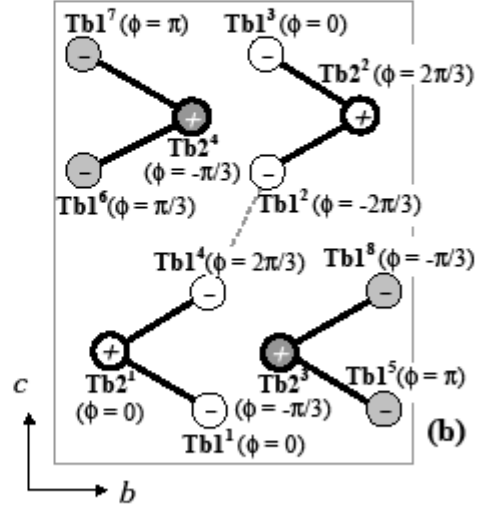
Figure 9. (a) Magnetic structure of Tb 3 Ni 2 Ge 3 below ~33 K and down to 17 K and (b) additional low-temperature magnetic component in the Tb 3 Ni 2 Ge 3 magnetic structure (from 15 K and down to 1.5 K). The shortest Tb1-Tb1 and Tb1-Tb2 interatomic distances are shown in Figure.
