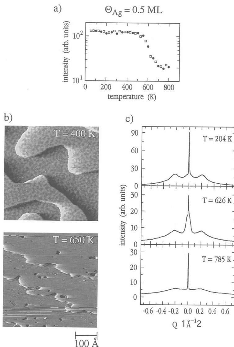
Fig. 2. Intensity (peak height) of the specularly reflected He-beam (a), He diffraction spectra (c) and STM topographs ( 450 \text{ Å} \times 450 \text{ Å} ) of the Ag-Pt(111) mixture for \Theta_{\text{Ag}} = 0.5 \text{ ML} (striped phase) taken at different temperatures (b). Open and filled symbols in (a) correspond to measurements taken during increasing and decreasing the surface temperature, respectively. The He-diffraction profiles in (c) were recorded along the [112]-direction using a He-beam energy of 21.6 meV and fixed total scattering angle ( \vartheta_i + \vartheta_f = 90^\circ ).
