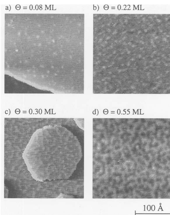
Fig. 1. Constant-current STM topographs ( 225 \text{ Å} \times 225 \text{ Å} ) of a Pt(111) surface after deposition of submonolayer amounts of Ag annealed at elevated temperatures ( T > 700 \text{ K} ), and imaged at 400 K: (a) Ag-coverage: \Theta_{\text{Ag}} = 0.08 \text{ ML} , annealing temperature: T = 700 \text{ K} ; (b) \Theta_{\text{Ag}} = 0.22 \text{ ML} , T = 850 \text{ K} ; (c) \Theta_{\text{Ag}} = 0.30 \text{ ML} , T = 800 \text{ K} ; (d) \Theta_{\text{Ag}} = 0.55 \text{ ML} , T = 850 \text{ K} . Note that in taking (b) and (c) a high-pass filter was used which enhances the contrast for steep changes of the tip-height. (a) and (d) are regular grey-scale images of the tip-height.
