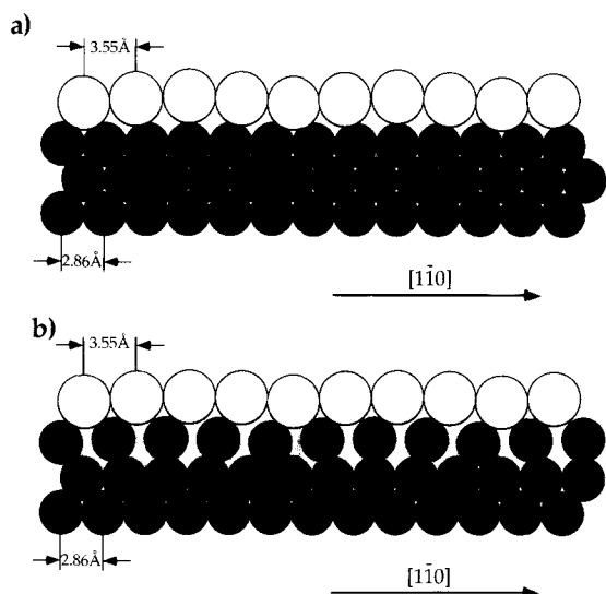
Fig. 11. Structure models: (a) Simple adlayer of S atoms (large white circles) on the Al substrate (smaller gray circles). (b) Bilayer consisting of S atoms and an expanded layer of Al atoms (dark gray circles).
