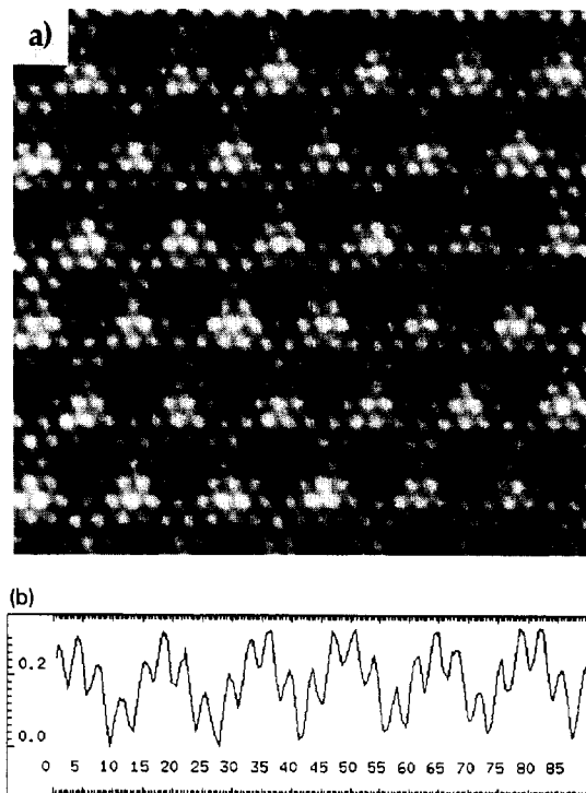
Fig. 1. (a) STM topograph of the non-rotated adlayer; (b) profile along a close-packed row. 92 \text{ Å} \times 87 \text{ Å} , I = 0.3 \text{ nA} , V = -0.2 \text{ V} , T_{\text{ads}} = 570 \text{ K} , 330 L H_2S .
