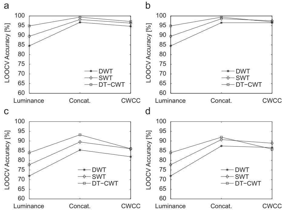
Fig. 5. Visualization of differences in the LOOCV accuracies between the luminance-channel results and the results of both combining schemes for J = 6 . (a) 2-Class, RGB, (b) 2-Class, LAB, (c) 6-Class, RGB, (d) 6-Class, LAB.
