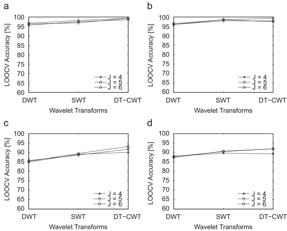
Fig. 3. Visualization the LOOCV accuracies for the feature vector concatenation combining scheme. (a) 2-Class, RGB, (b) 2-Class, LAB, (c) 6-Class, RGB, (d) 6-Class, LAB.
