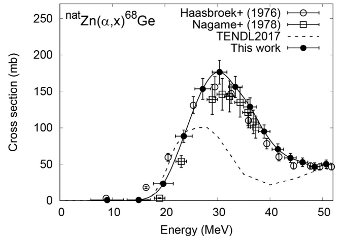
Fig. 2. Measured excitation function of the ^{nat}Zn(\alpha, x)^{68}Ge reaction. The result is compared with the previous experimental data [9,10] and the TENDL-2017 data [16].
