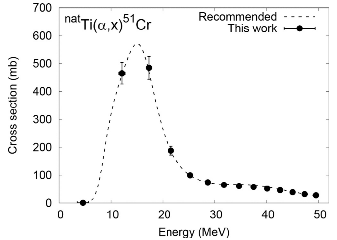
Fig. 1. Measured excitation function of the monitor ^{nat}Ti(\alpha, x)^{51}Cr reaction in comparison with the recommended values [15].
