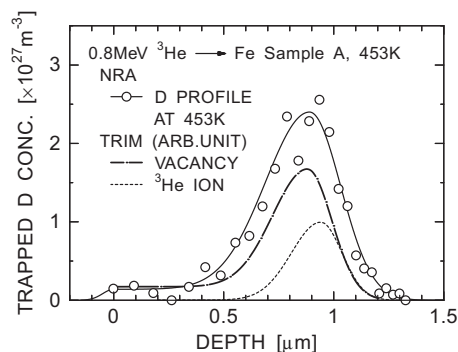
Fig. 2. Depth profile of trapped deuterium in Fe sample irradiated with 0.8-MeV ^3\text{He} . Distributions of vacancies and ^3\text{He} ions estimated using the TRIM code are also shown in arbitrary units.
