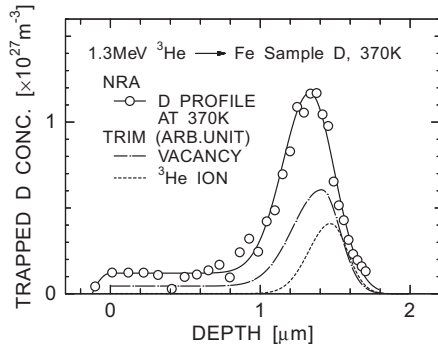
Fig. 3. Depth profile of trapped deuterium in Fe sample irradiated with 1.3-MeV ^3\text{He} . Distributions of vacancies and ^3\text{He} ions are also shown in arbitrary units.
