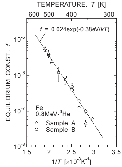
Fig. 5. Equilibrium constant for partitioning of deuterium between the trap and the solution site in ^3\text{He} -irradiated Fe.
