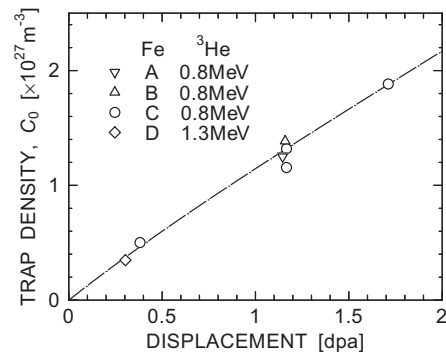
Fig. 6. Evolution of the trap density with atomic displacement in ^3\text{He} -irradiated Fe.
