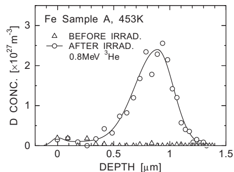
Fig. 1. Deuterium depth profiles of Fe sample at 453 K before and after irradiation with 0.8-MeV ^3\text{He} ions.
