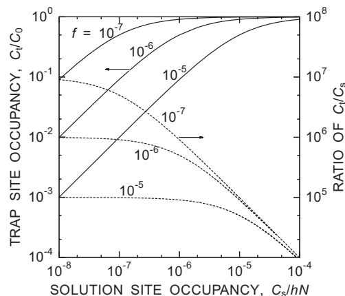
Fig. 7. Dependence of the trap site occupancy, C_t/C_0 , and the concentration ratio, C_t/C_s , on the solution site occupancy, C_s/hN .
