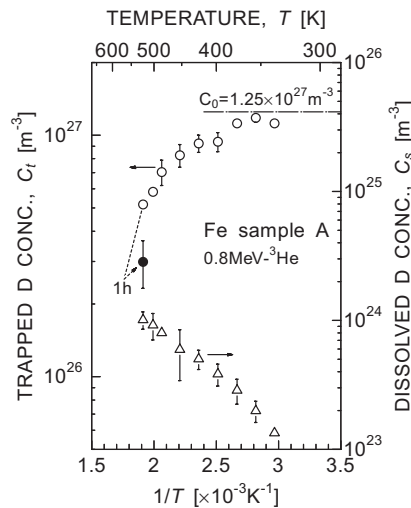
Fig. 4. Temperature dependence of the deuterium concentration in the trap, C_t , and in the solution site, C_s , for sample A. A filled symbol represents the C_t after annealing at 568 K for 1 h.
