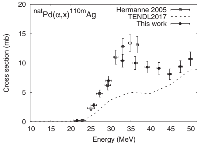
Fig. 8. The excitation function of the ^{nat}\text{Pd}(\alpha,x)^{110m}\text{Ag} reaction.
