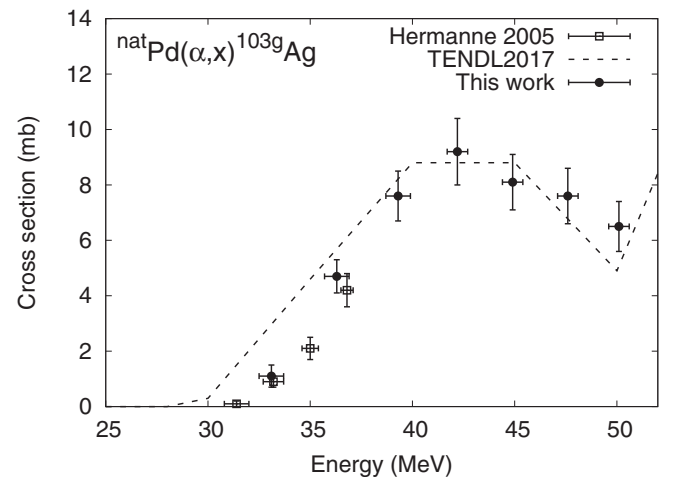
Fig. 11. The excitation function of the ^{nat}\text{Pd}(\alpha,x)^{103g}\text{Ag} reaction.
