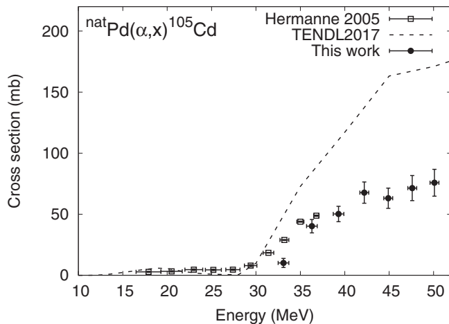
Fig. 5. The excitation function of the ^{nat}\text{Pd}(\alpha, x)^{105}\text{Cd} reaction.
