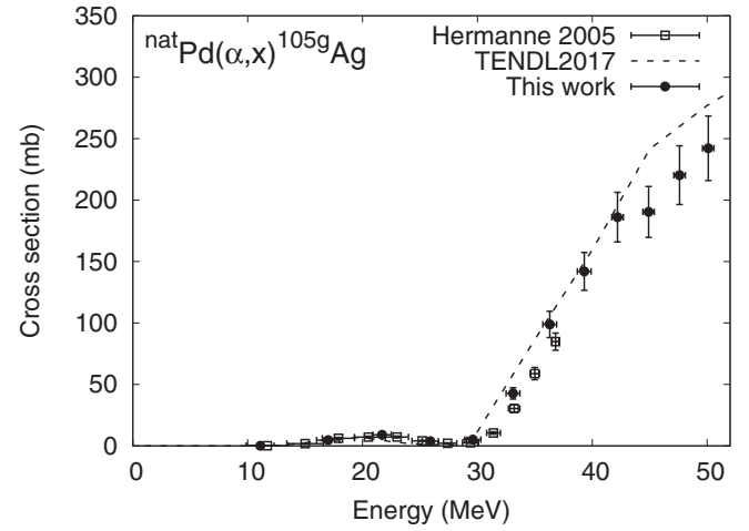
Fig. 10. The excitation function of the ^{nat}\text{Pd}(\alpha,x)^{105g}\text{Ag} reaction.
