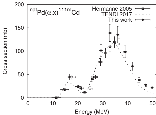
Fig. 2. The excitation function of the ^{nat}\text{Pd}(\alpha,x)^{111m}\text{Cd} reaction.
