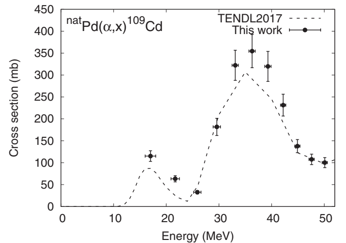
Fig. 3. The excitation function of the ^{nat}\text{Pd}(\alpha,x)^{109}\text{Cd} reaction.
