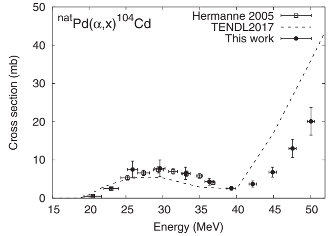
Fig. 6. The excitation function of the ^{nat}\text{Pd}(\alpha, x)^{104}\text{Cd} reaction.
