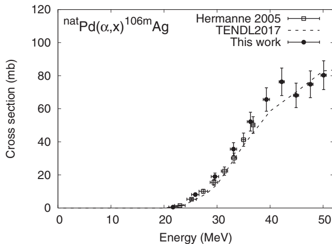
Fig. 9. The excitation function of the ^{nat}\text{Pd}(\alpha,x)^{106m}\text{Ag} reaction.
