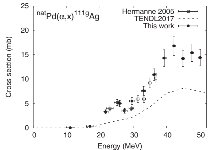
Fig. 7. The excitation function of the ^{nat}\text{Pd}(\alpha, x)^{111g}\text{Ag} reaction.
