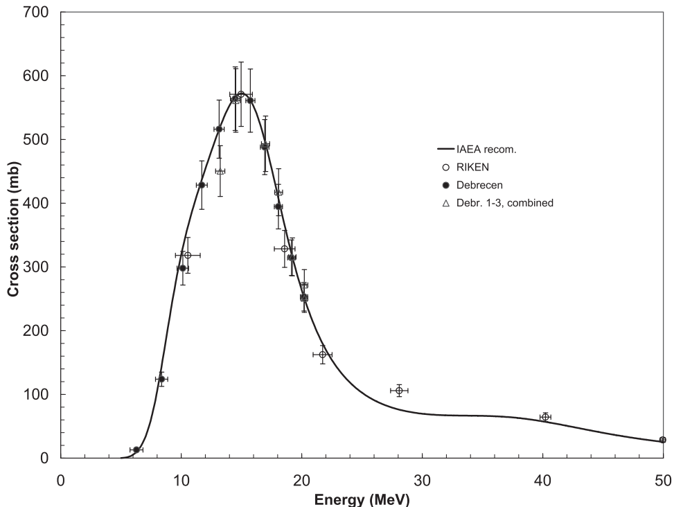
Fig. 1. Comparison of the recommended excitation function of the ^{nat}\text{Ti}(\alpha, x)^{51}\text{Cr} reaction [21] and the experimental cross section data points deduced in these experiments. The open circle represents the experiment in RIKEN, the full dot represents the stack in Atomki containing only Ti foils, and the open triangle represents the combined three experiments in Atomki with Ge targets.
