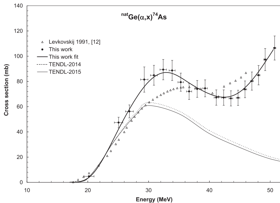
Fig. 7. Experimental cross section data for the {}^{\text{nat}}\text{Ge}(\alpha, x){}^{74}\text{As} reaction in comparison with the earlier measured data and the result of the theoretical calculations. The thick solid line is a spline fit over the experimental points measured in this work.
