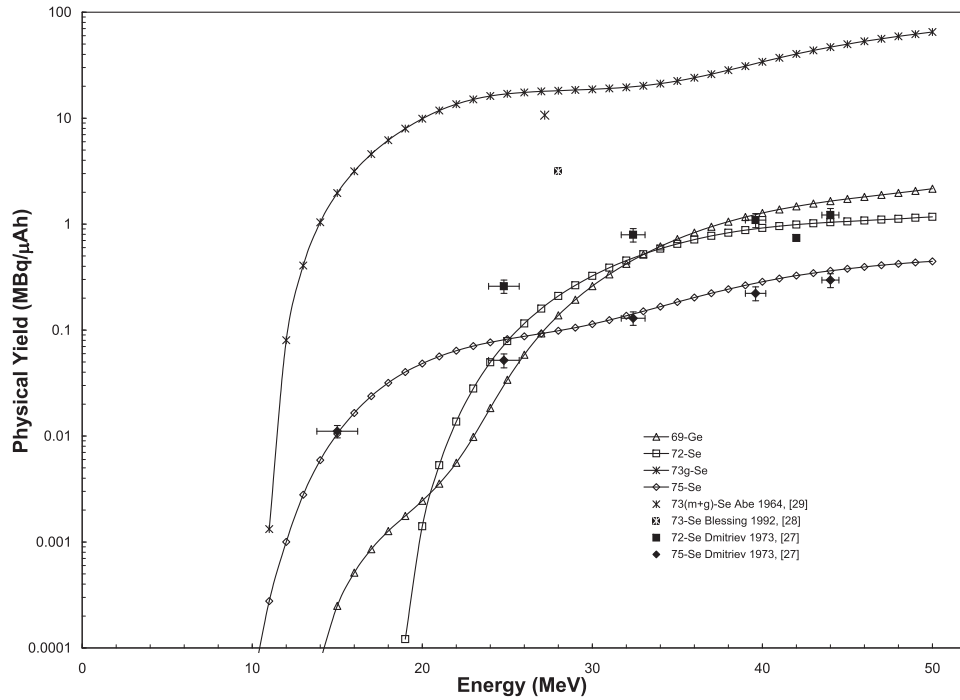
Fig. 11. Calculated physical thick target yields for production of ^{72,73,75}\text{Se} and ^{69}\text{Ge} based on the newly measured cross section data in comparison with the available experimental yield data.
