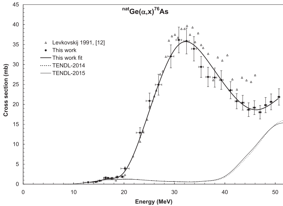
Fig. 8. Experimental cross section data for the ^{nat}\text{Ge}(\alpha, x)^{76}\text{As} reaction in comparison with the earlier measured data and the result of the theoretical calculations. The thick solid line is a spline fit over the experimental points measured in this work.
