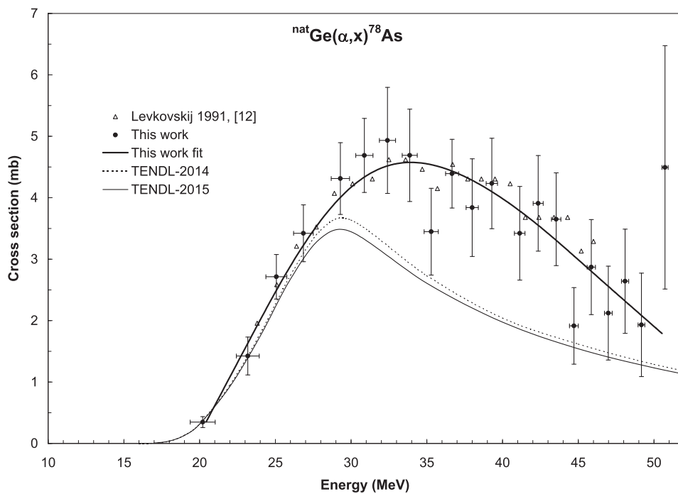
Fig. 9. Experimental cross section data for the ^{nat}\text{Ge}(\alpha, x)^{78}\text{As} reaction in comparison with the earlier measured data and the result of the theoretical calculations. The thick solid line is a spline fit over the experimental points measured in this work.
