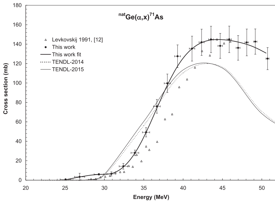
Fig. 5. Experimental cross section data for the {}^{\text{nat}}\text{Ge}(\alpha, x){}^{71}\text{As} reaction in comparison with the earlier measured data and the result of the theoretical calculations. The thick solid line is a spline fit over the experimental points measured in this work.
