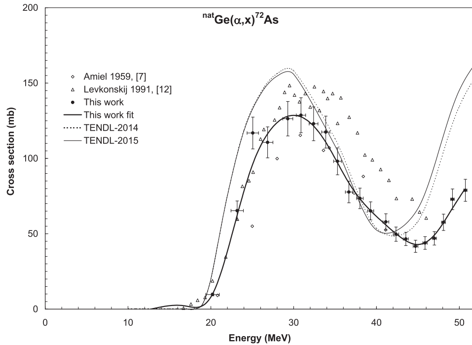
Fig. 6. Experimental cross section data for the {}^{\text{nat}}\text{Ge}(\alpha, x){}^{72}\text{As} reaction in comparison with the earlier measured data and the result of the theoretical calculations. The thick solid line is a spline fit over the experimental points measured in this work.
