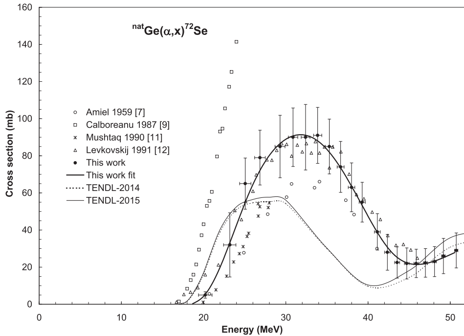
Fig. 2. Experimental cross section data for the {}^{\text{nat}}\text{Ge}(\alpha, x){}^{72}\text{Se} reaction in comparison with the earlier measured data and the results of theoretical calculations. The thick solid line is a spline fit over the experimental points measured in this work.
