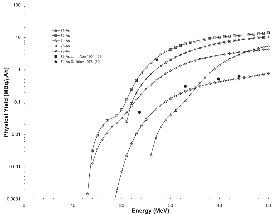
Fig. 12. Calculated physical thick target yields for production of ^{71,72,74,76,78}\text{As} based on the newly measured cross section data in comparison with the available experimental yield data.
