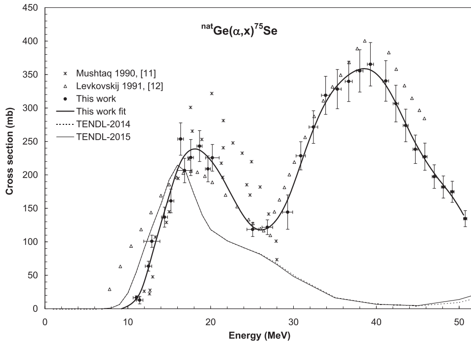
Fig. 4. Experimental cross section data for the {}^{\text{nat}}\text{Ge}(\alpha, x){}^{75}\text{Se} reaction in comparison with the earlier measured data and the result of the theoretical calculations. The thick solid line is a spline fit over the experimental points measured in this work.
