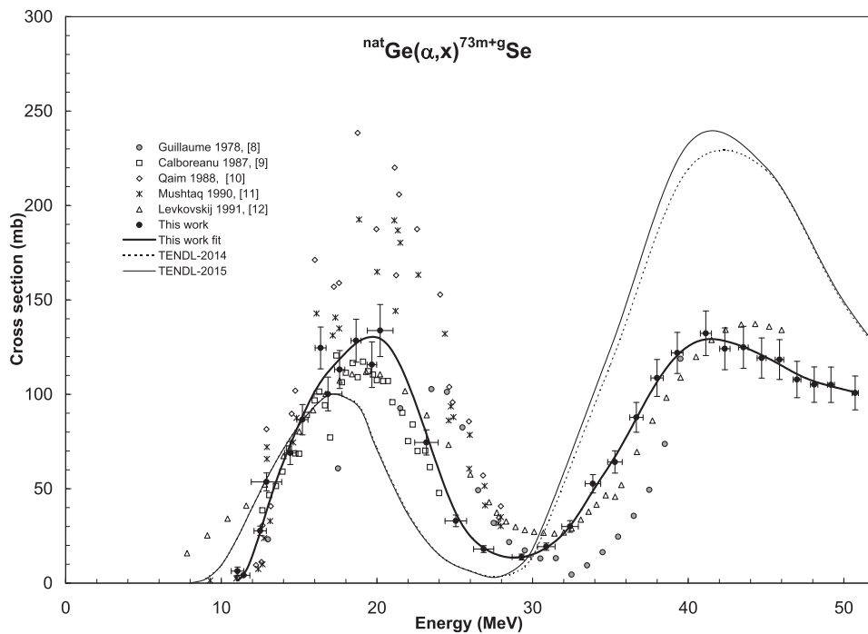
Fig. 3. Experimental cross section data for the {}^{\text{nat}}\text{Ge}(\alpha, x){}^{73\text{m}+\text{g}}\text{Se} reaction in comparison with the available literature data and the result of the theoretical calculations. The thick solid line is a spline fit over the experimental points measured in this work.
