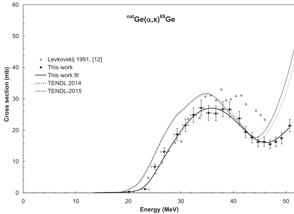
Fig. 10. Experimental cross section data for the {}^{\text{nat}}\text{Ge}(\alpha, x){}^{69}\text{Ge} reaction in comparison with the earlier measured data and the result of the theoretical calculations. The thick solid line is a spline fit over the experimental points measured in this work.
