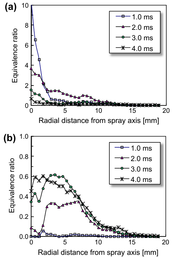
Fig. 9. Temporal variations of equivalence ratio distributions along radial direction from spray axis ( T_a = 500 K, P_a = 1.0 MPa, fuel: p-xylene, z = 25 mm). (a) liquid phase. (b) vapor phase.
