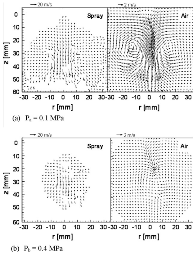
Fig. 7. Velocity distributions of spray droplets and spray-induced ambient air flow ( T_a = 300 K, t = 3 ms ASOI, fuel: dry solvent).
