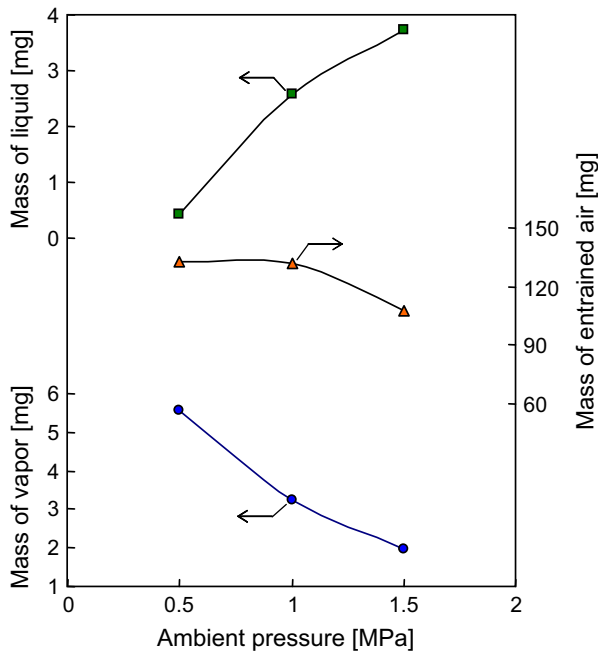
Fig. 12. Effect of ambient pressure on mass of liquid, vapor and entrained air in the spray ( T_a = 500 K, t = 3 ms ASOI, fuel: p-xylene).
