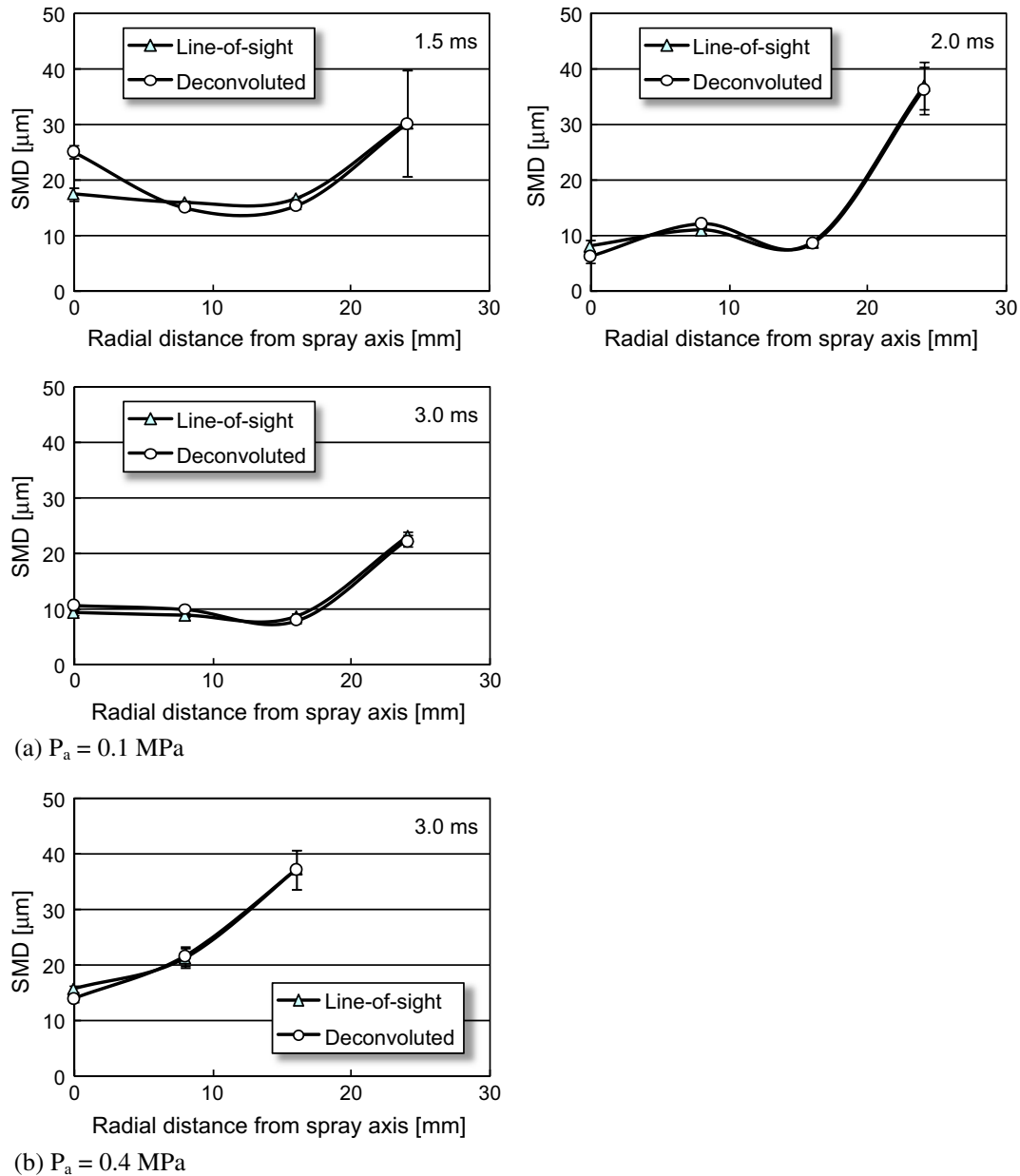
Fig. 6. Spatial droplet size distribution ( T_a = 300 K, fuel: dry solvent, r = 0 mm, z = 30 mm).
