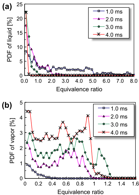
Fig. 10. Temporal variations of probability density function (PDF) of equivalence ratio in the (a) liquid and (b) vapor phase sprays ( T_a = 500 K, P_a = 1.0 MPa, fuel: p-xylene).
