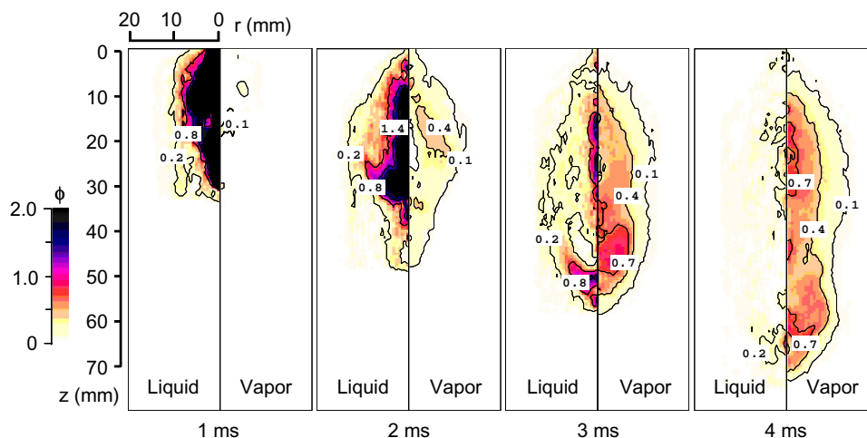
Fig. 8. Temporal variations of spatial equivalence ratio distributions of liquid and vapor phases in the spray ( T_a = 500 K, P_a = 1.0 MPa, fuel: p-xylene).
