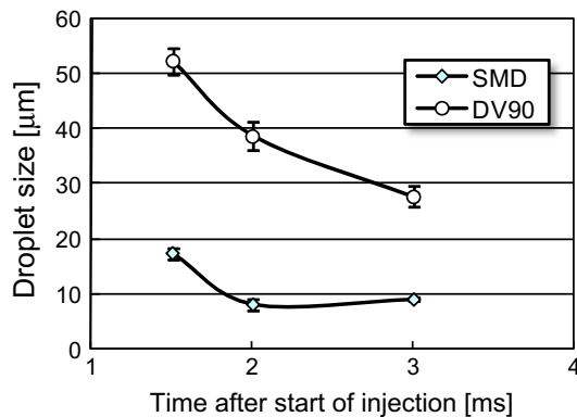
(a) P_a = 0.1 MPa
