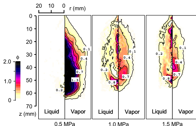
Fig. 11. Effect of ambient pressure on spatial equivalence ratio distributions of liquid and vapor phases in the spray ( T_a = 500 K, t = 3 ms ASOI, fuel: p-xylene).
