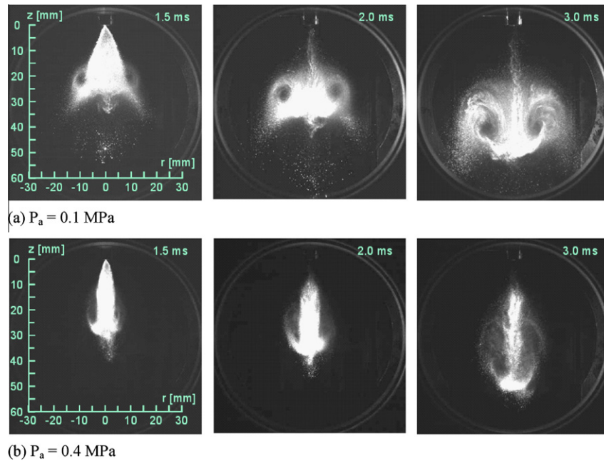
Fig. 4. Mie scattering images of spray droplets by laser sheet method ( T_a = 300 K, fuel: dry solvent).
