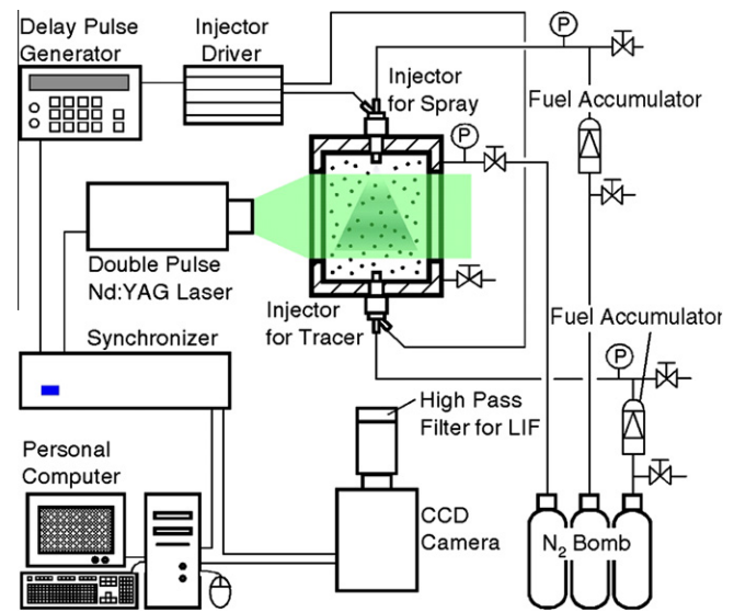
Fig. 2. Schematic of experimental apparatus for LIF-PIV and laser sheet imaging.
