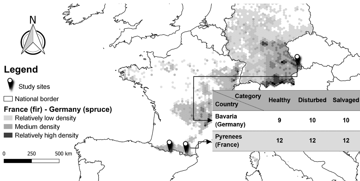
Fig. 1. Map showing the study sites in Germany (Bavaria) and in France (Pyrenees) and the number of plots for each country and each stand category. Mapping was performed in QGIS 3.10. Hexagonal binning was based on GBIF data for Abies alba in France and for Picea abies in Germany (GBIF.org, 2020).
