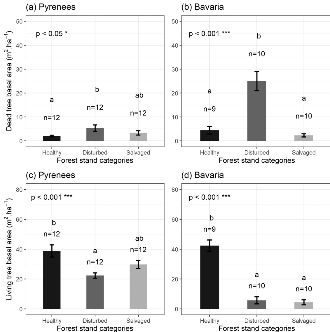
Fig. 2. Basal area ( \text{m}^2 \text{ha}^{-1} ) of dead trees (a, b) and living trees (c, d) in the 0.3-ha plots for each country and each stand category. Dead trees (snags) more than 7.5 cm in diameter are included. Letters indicate significant differences between each category (p value top-left). The letters result from post-hoc Tukey tests on generalized (negative binomial) linear mixed models.
