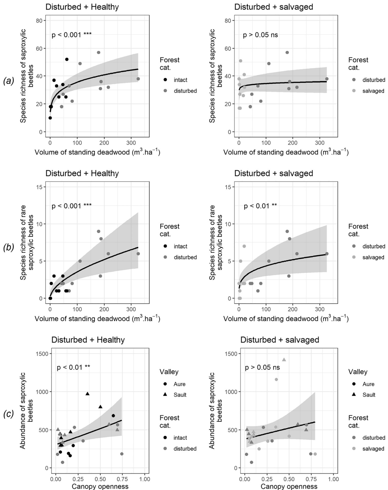
Fig. 7. Relationship between standing deadwood volume in Bavarian spruce forests and mean species richness of saproxylic beetles (a), or red-listed saproxylic beetles (b), and between canopy openness in Pyrenean silver fir forests and mean abundance of all saproxylic beetles (c). Left: disturbed and “intact” (or healthy) stands; Right: disturbed and salvaged stands. The black line is the regression curve from the negative binomial model (with a log-transformation of x) and the grey area indicates the 95% confident interval. “intact” = “healthy”.
