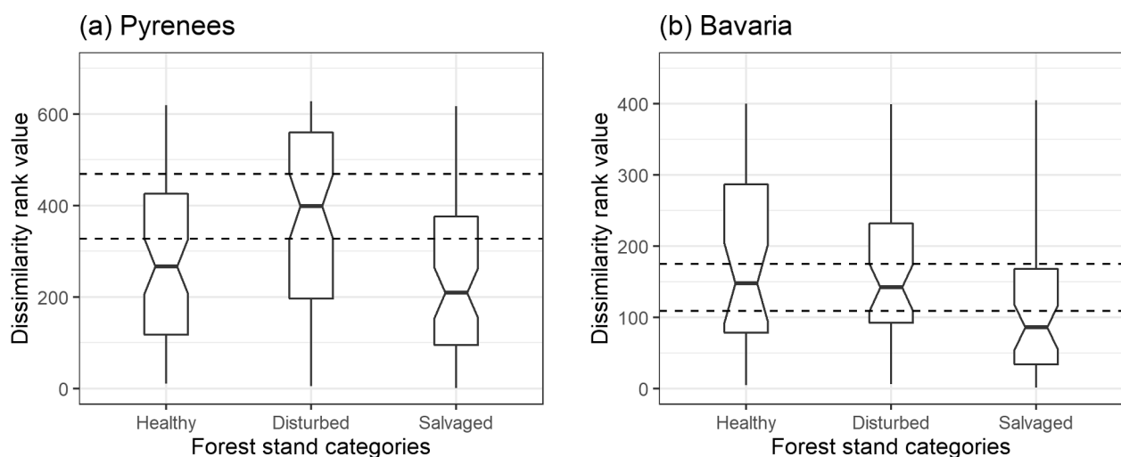
Fig. 5. ANOSIM plots showing the dissimilarity among beetle assemblages within the given forest stand categories in the Pyrenees (left) and in Bavaria (right). The bold horizontal bar in the box indicates the median; the bottom of the box indicates the 25th percentile; the top of the box indicates the 75th percentile and the extreme data points are marked by whiskers. Notches are used to differentiate group medians: if the notches for two boxes do not overlap, this is strong evidence that two medians differ (Chambers et al., 2018). Dotted lines indicate lower and upper notches from the disturbed category for comparison with the healthy and salvaged categories.
