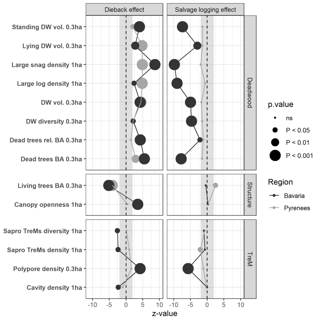
Fig. 3. Response of local forest stand features (deadwood, stand structure and tree-related microhabitats) to tree dieback (left panels) and salvage logging (right panels) in the Bavarian spruce forests (black) and in the Pyrenean silver fir forests (grey). Circles indicate effect significance and their diameter varies with p-value (lines between points are for visual purposes only); shaded areas indicate the range of non-significant values (z-values: \pm 2.0 ).
