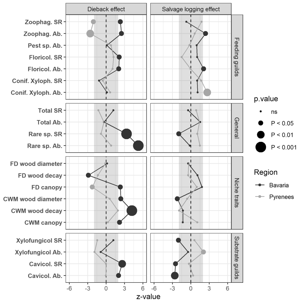
Fig. 4. Response of local saproxylic beetle community metrics (feeding guilds, niche trait guilds, substrate guilds and general diversity metrics) to tree dieback (left panels) and salvage logging (right panels) in Bavarian spruce forests (black) and in Pyrenean silver fir forests (grey). Circles indicate effect significance and their diameter varies with p-value (lines between points are for visual purposes only); shaded areas indicate the range of non-significant values (z-values: \pm 2.0 ).
