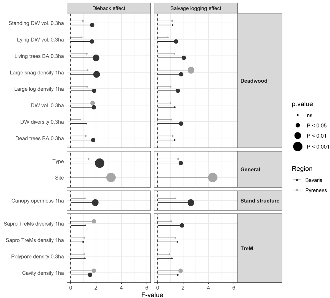
Fig. 6. Environmental drivers of variations in saproxylic beetle species composition, associated to tree dieback or salvage logging effects in Bavarian spruce forests (black) and in Pyrenean silver fir forests (grey). Effects of local stand features (deadwood, stand structure and tree-related microhabitats) tested with Canonical Analysis of Principal coordinates based on Bray-Curtis distance matrices: total inertia explained by each variable including inertia co-explained with other variables (bottom panel). Circles indicate effect significance and their diameter varies with p-value (100-run permutation tests).
