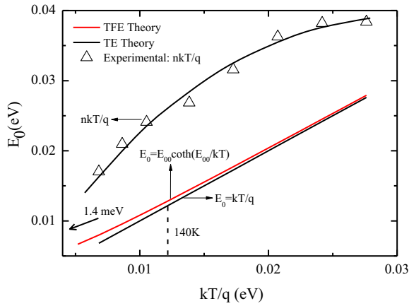
Fig. 4. E_0 as a function of temperature calculated using Eqs. (3) (TE) and (6) (TFE) respectively compared to the experimental values for E_0 .
