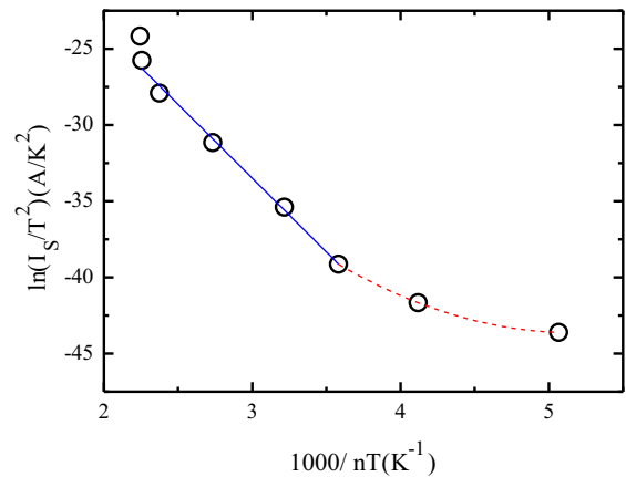
Fig. 6. An adjusted Richardson plot as expressed in Eq. (7). The non-ideal nature of the Pd/n-GaSb SBDs has been taken into account.
