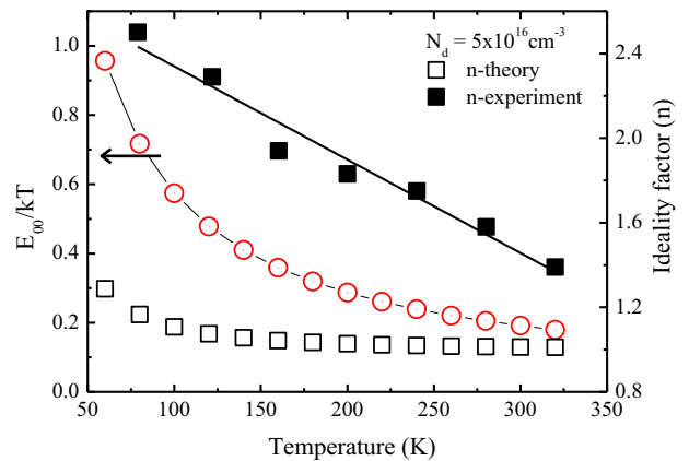
Fig. 1. E_{00}/kT values as a function of temperature (open circles) and a comparison between the theoretically determined (assuming TFE — open squares) and experimentally obtained (solid squares) ideality factors.
