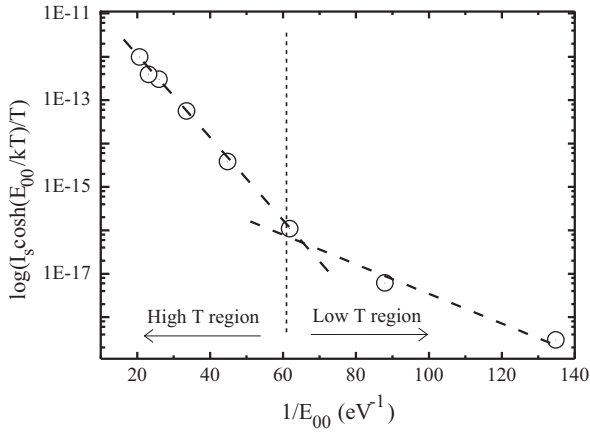
Fig. 7. The measured saturation current plotted against the tunnelling factor 1/E_0 for the Pd/n-GaSb structure studied. Note the possibility of a second, much lower barrier height in the low temperature region.
