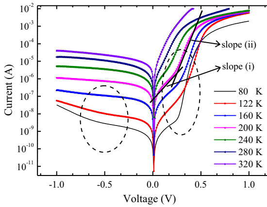
Fig. 2. Current–voltage characteristics of a Pd/n-GaSb Schottky contact in the temperature range of 80–320 K.
