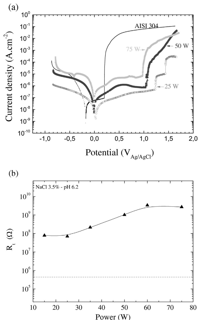
Fig. 10. (a) Potentiodynamic polarization curves and (b) total resistance of the systems coated with films of different thicknesses as a function of the plasma excitation power. The dotted line represents the total resistance for the untreated steel substrate.
