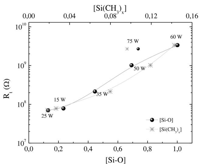
Fig. 12. Total resistance of the systems containing films with different thicknesses as a function of the relative density of SiO and Si(CH 3 ) x .
