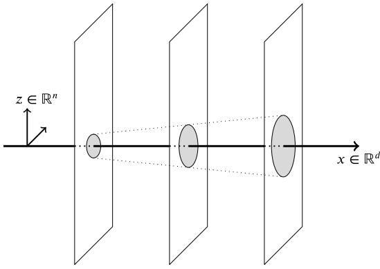
Fig. 1. Particle-wave interactions.
