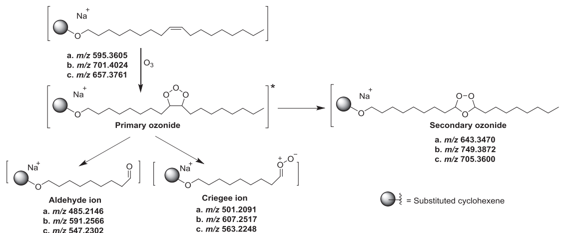
Fig. 4. Proposed mechanism for OzID fragmentation of 1–3 (a–c) [Criegee ion (representative structure shown but isomers of the carbonyl oxide cannot be excluded)].
