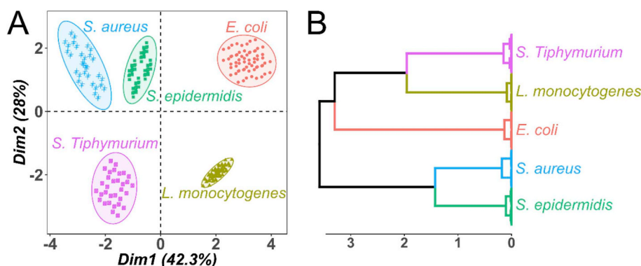
Fig. 2. Multivariate data analyses for 5 bacterial strains processed on AMP-arrays. (A) 2D-score plot of the database generated from the kinetics of SPRI bacterial growth monitoring. Ellipses were annotated to represent the 95% confidence interval. (B) Hierarchical Clustering on Principal Components (HCPC) performed on the data from Fig. 2a. Distances between points are Euclidean.
