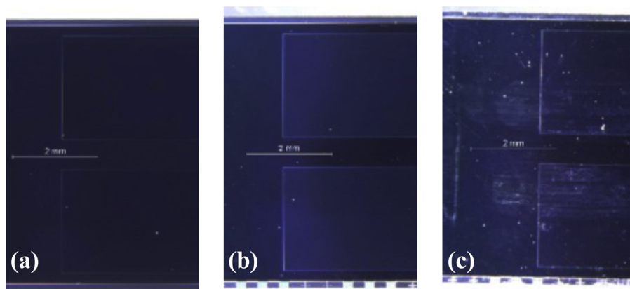
Fig. 2. Magnified photograph of a brand new chip (a), a reused chip applying the optimized regeneration protocol (b) and a chip rinsed with water and isopropanol (c).
