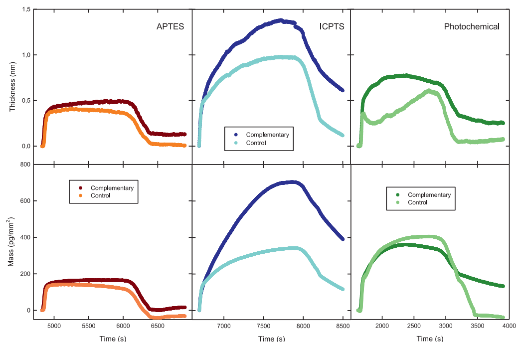
Fig. 3. Evolution of thickness (top) and mass (bottom) with time during the hybridization step. Comparison between the different probe immobilization modes. Gelatine was employed as blocking agent in all cases.
