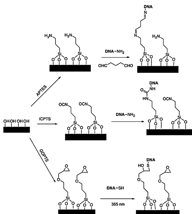
Fig. 1. Scheme of the chemical processes taking place on the chip surface.
