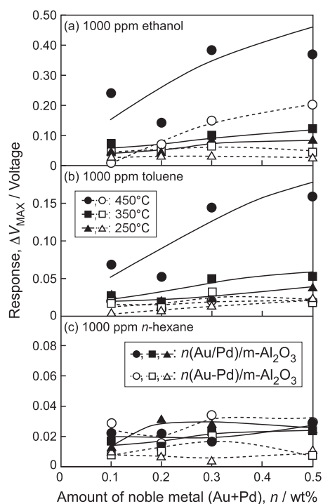
Fig. 12. Variations in the \Delta V_{\text{MAX}} to 1000 ppm ethanol, toluene and n -hexane in air with the amount of Au and Pd loaded ( n ) of n(\text{Au/Pd})/\text{mp-Al}_2\text{O}_3 and n(\text{Au-Pd})/\text{mp-Al}_2\text{O}_3 sensors.
