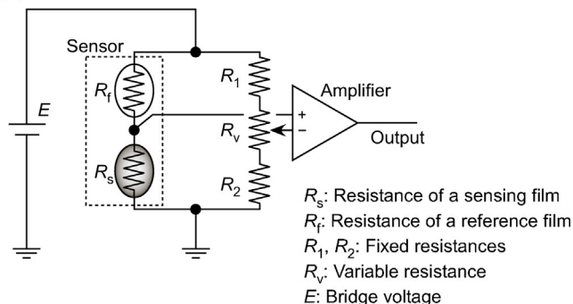
Fig. 1. (a) Schematic drawing of an adsorption/combustion-type gas sensor and (b) a bridge circuit containing the micro-sensor chip.
