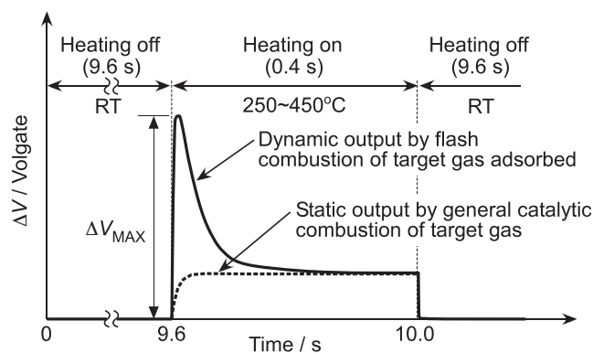
Fig. 2. Typical sensor-signal profile of adsorption/combustion-type gas sensors. \Delta V (vertical axis): the difference between output voltage in a target gas ( V_g ) and that in air ( V_a ).
