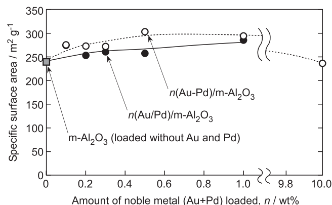
Fig. 6. Variation in SSA of all n(\text{Au-Pd})/\text{mp-Al}_2\text{O}_3 and n(\text{Au-Pd})/\text{mp-Al}_2\text{O}_3 powders prepared in this study, with the amount of noble metal (Au + Pd) loaded.
