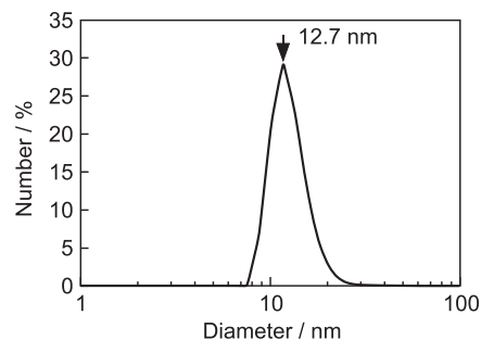
Fig. 3. Particle-size distribution of Au/Pd nanoparticles synthesized in this study.
