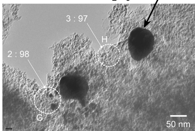
Fig. 8. TEM photographs of 1.0(Au/Pd)/mp-Al 2 O 3 and 1.0(Au-Pd)/mp-Al 2 O 3 powders heat-treated at 700 °C for 2 h in air, together with the ratio of Au to Pd (Au:Pd) of some regions in weight.
