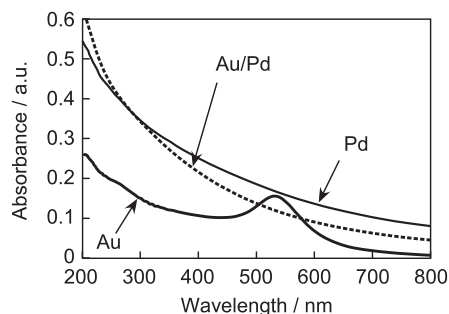
Fig. 5. UV-vis absorption spectrum of Au/Pd nanoparticles synthesized in this study.
