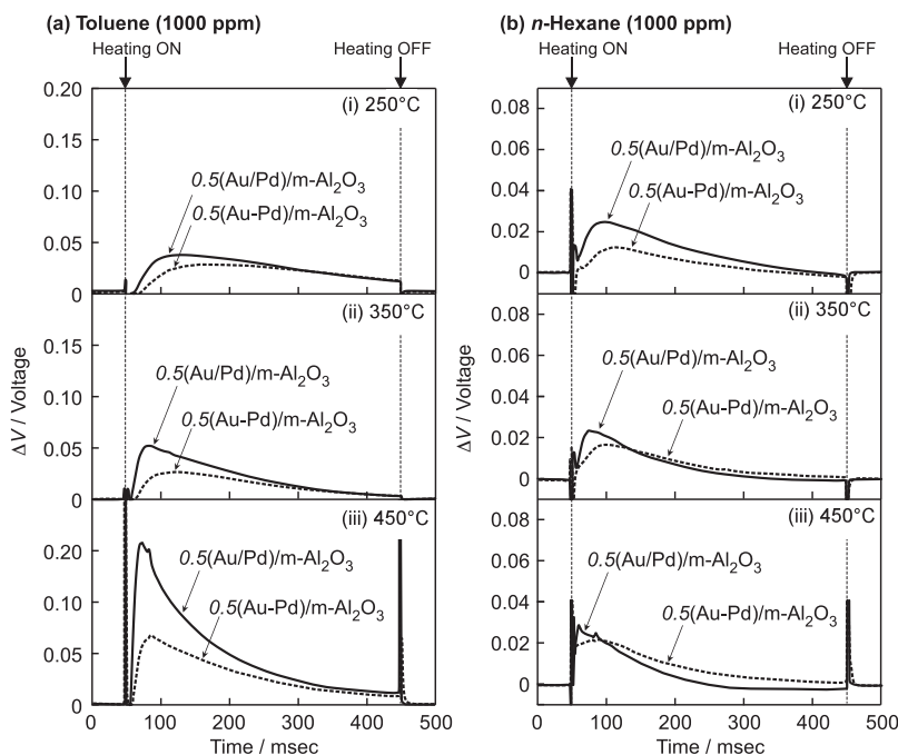
Fig. 11. Sensor-signal profiles to 1000 ppm toluene and n -hexane of 0.5(\text{Au/Pd})/\text{mp-Al}_2\text{O}_3 and 0.5(\text{Au-Pd})/\text{mp-Al}_2\text{O}_3 sensors in air at the pulse-heating temperature of 250–450 °C.
