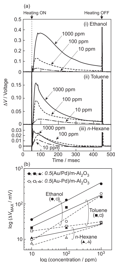
Fig. 13. (a) Sensor-signal profiles of the 0.5(\text{Au/Pd})/\text{mp-Al}_2\text{O}_3 sensor to 10, 100 and 1000 ppm ethanol, toluene and n -hexane and (b) dependence of logarithmic \Delta V_{\text{MAX}} of 0.5(\text{Au/Pd})/\text{mp-Al}_2\text{O}_3 and 0.5(\text{Au-Pd})/\text{mp-Al}_2\text{O}_3 sensors on concentration of ethanol, toluene and n -hexane in air at the pulse-heating temperature of 450 °C.
