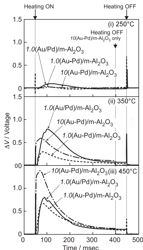
Fig. 9. Sensor-signal profiles of 1.0(Au/Pd)/mp-Al 2 O 3 and 1.0(Au-Pd)/mp-Al 2 O 3 sensors to 1000 ppm ethanol in air at the pulse-heating temperature of 250–450 °C, together with those of a 10(Au-Pd)/mp-Al 2 O 3 sensor.
