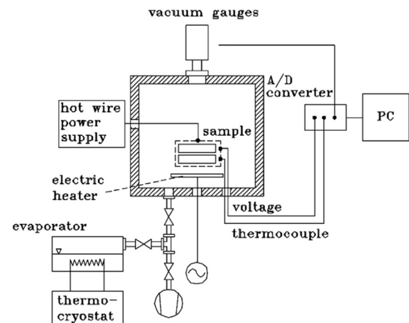
Fig. 8. Hot wire thermal conductivity measurement technique [37].
