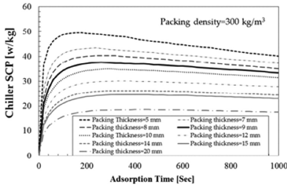
Fig. 18. Chiller SCP at various adsorbent thicknesses [80].
