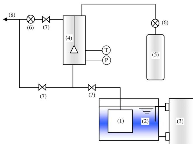
Fig. 12. TGA test facility [12].
