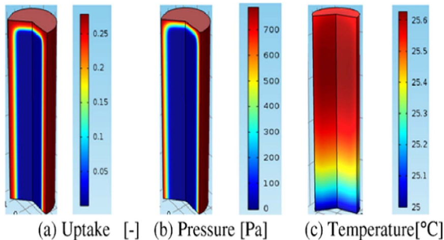
Fig. 20. Uptake, pressure, and temperature distribution in single adsorbent NX3/Ethanol particle at 400 s [107].
