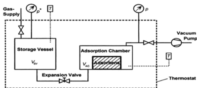
Fig. 10. Volumetric technique for measuring adsorption isotherms [76].
