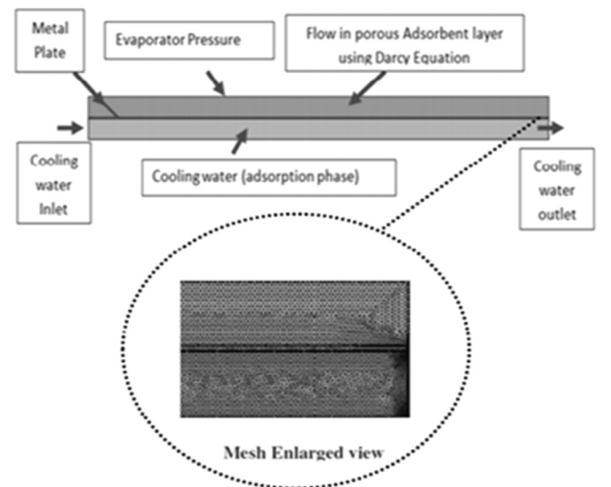
Fig. 17. Plate type adsorber configuration for the CFD modelling [80].
