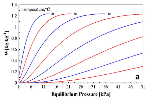
Maxsorb III/methanol [15]
