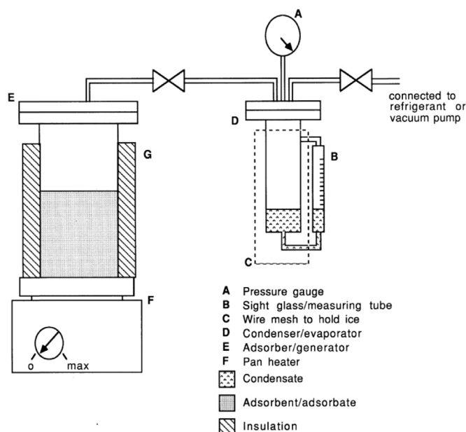
Fig. 15. Manual refrigerant liquid recording [88].
