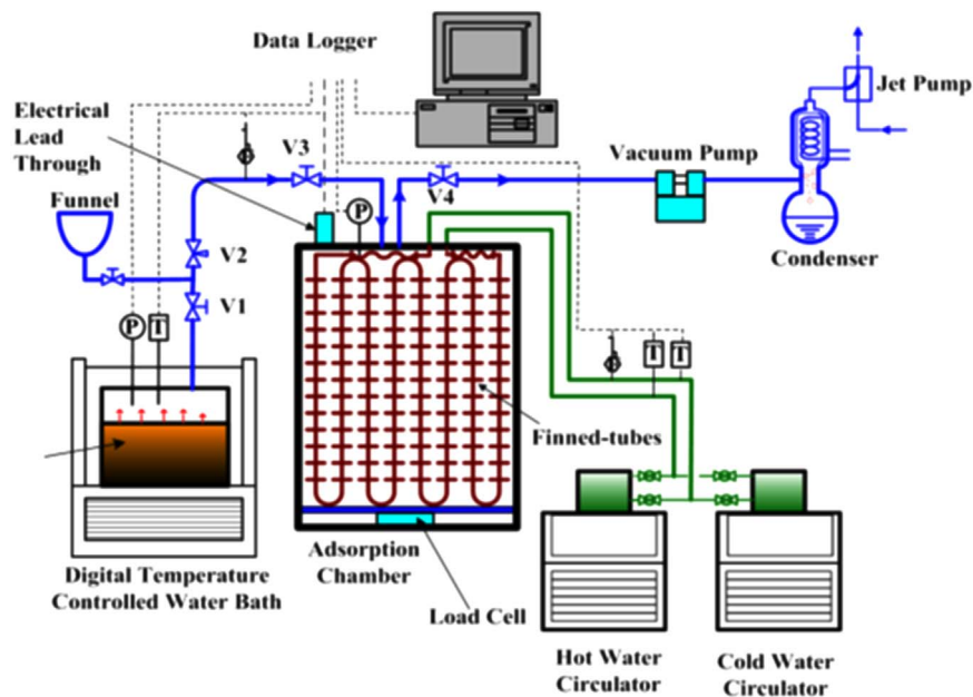
Fig. 13. Load cell sensor technique used by Ming [81].
