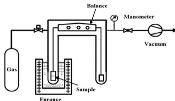
Fig. 11. Gravimetric concept of isotherm measurements [76].
